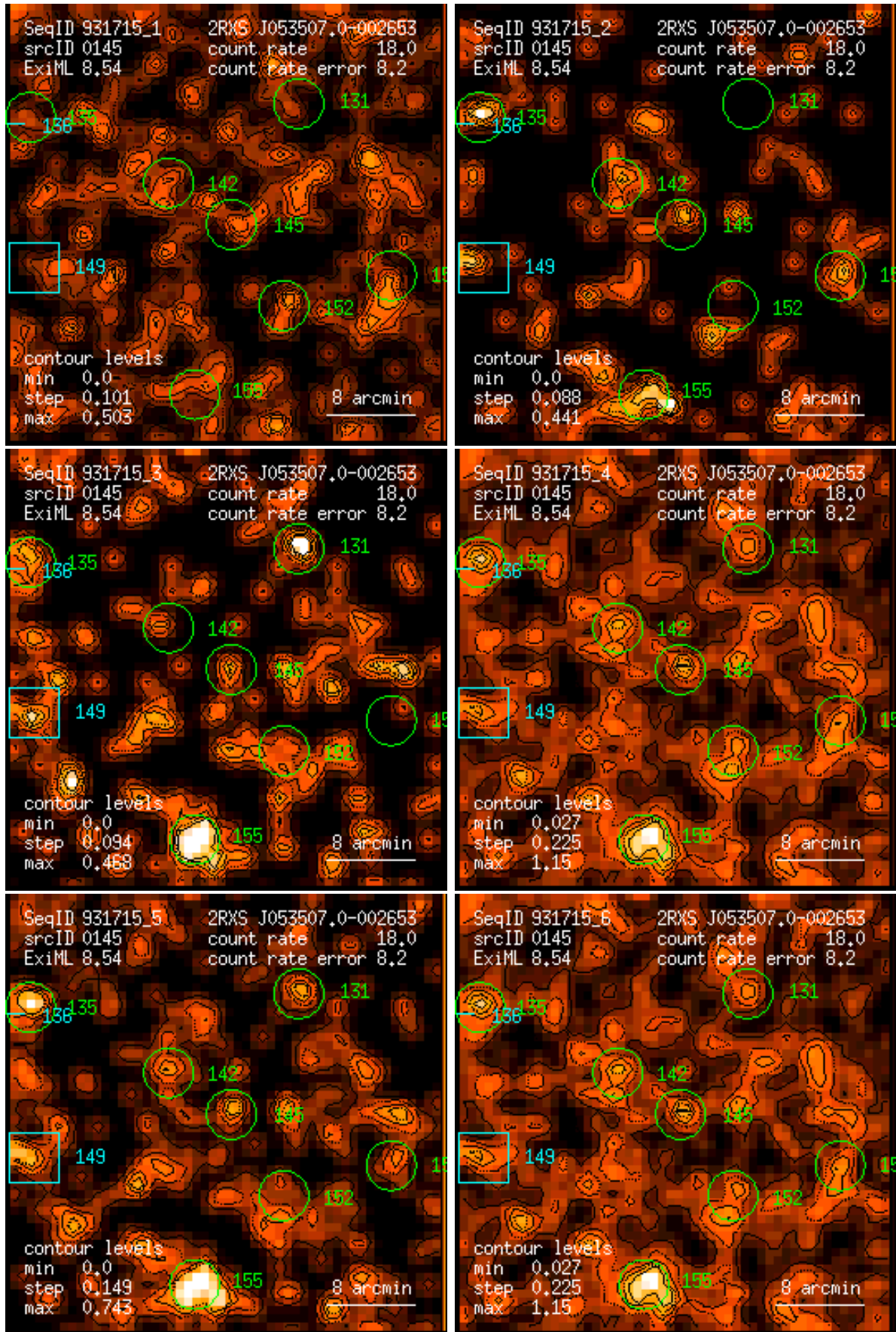
Figure 145: RASS 931715: detection 0145: band rate images, Gaussian filter: (1) PSPC channels 11 – 41, (2) 52 – 90, (3) 91 – 201, (4) 11 – 235, (5) 52 – 201, (6) 11 – 201. Broad band rates in counts/ks. Band rate contour levels in counts/ks/arcmin 2 .
