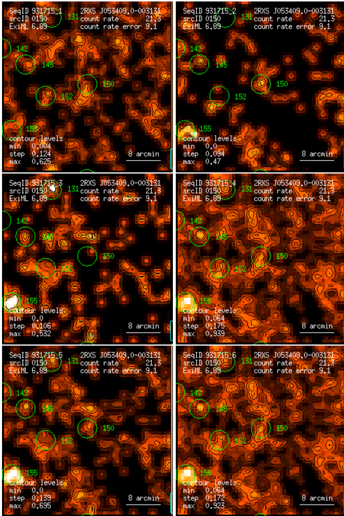
Figure 150: RASS 931715: detection 0150: band rate images, Gaussian filter: (1) PSPC channels 11 – 41, (2) 52 – 90, (3) 91 – 201, (4) 11 – 235, (5) 52 – 201, (6) 11 – 201. Broad band rates in counts/ks. Band rate contour levels in counts/ks/arcmin 2 .
