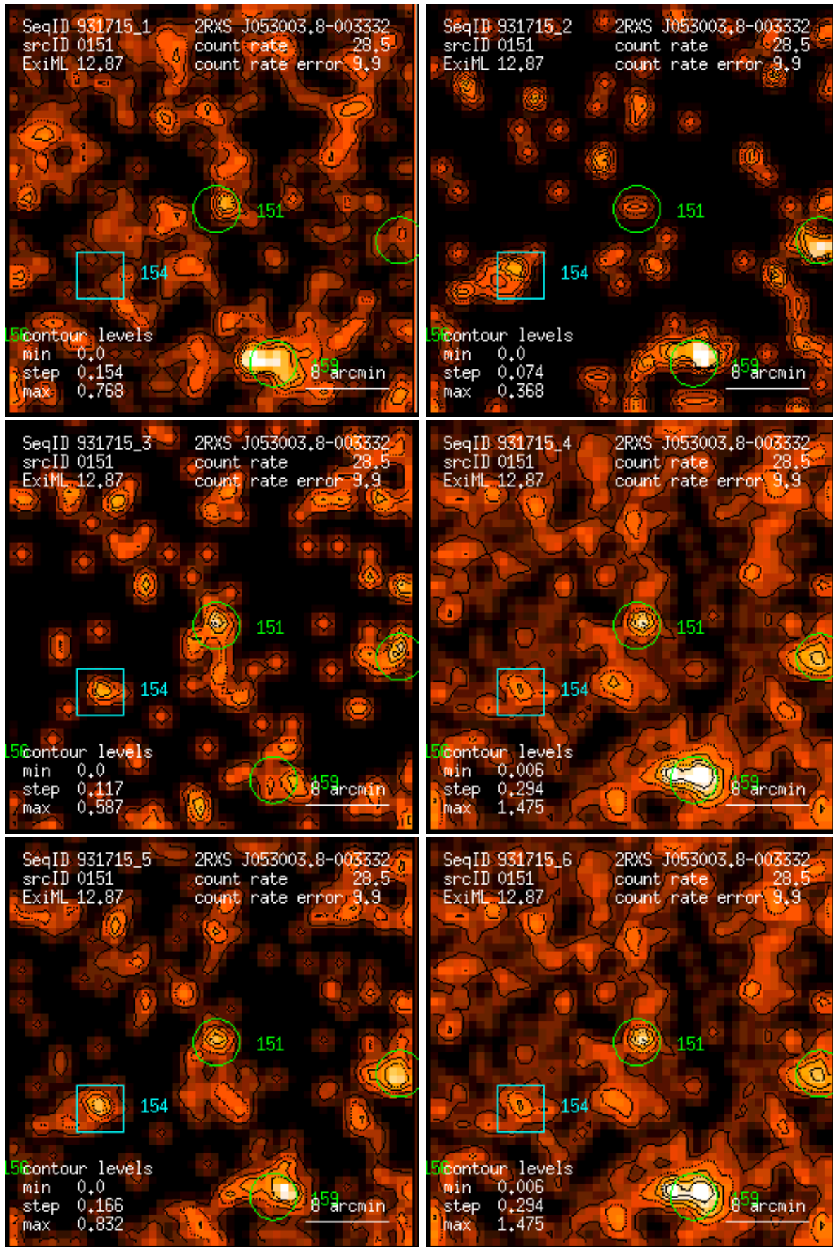
Figure 151: RASS 931715: detection 0151: band rate images, Gaussian filter: (1) PSPC channels 11 – 41, (2) 52 – 90, (3) 91 – 201, (4) 11 – 235, (5) 52 – 201, (6) 11 – 201. Broad band rates in counts/ks. Band rate contour levels in counts/ks/arcmin 2 .
