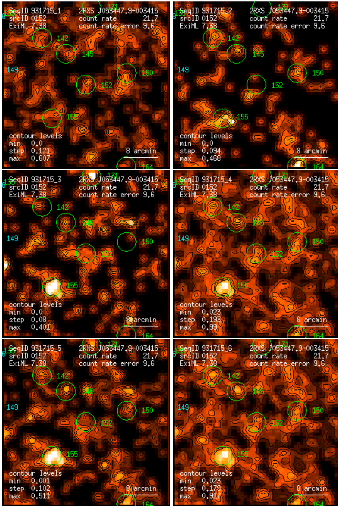
Figure 152: RASS 931715: detection 0152: band rate images, Gaussian filter: (1) PSPC channels 11 – 41, (2) 52 – 90, (3) 91 – 201, (4) 11 – 235, (5) 52 – 201, (6) 11 – 201. Broad band rates in counts/ks. Band rate contour levels in counts/ks/arcmin 2 .
