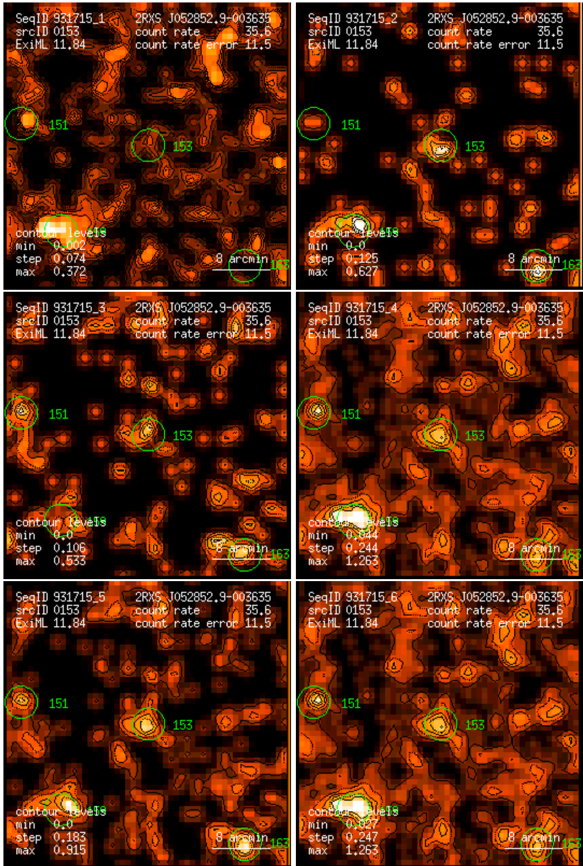
Figure 153: RASS 931715: detection 0153: band rate images, Gaussian filter: (1) PSPC channels 11 – 41, (2) 52 – 90, (3) 91 – 201, (4) 11 – 235, (5) 52 – 201, (6) 11 – 201. Broad band rates in counts/ks. Band rate contour levels in counts/ks/arcmin 2 .
