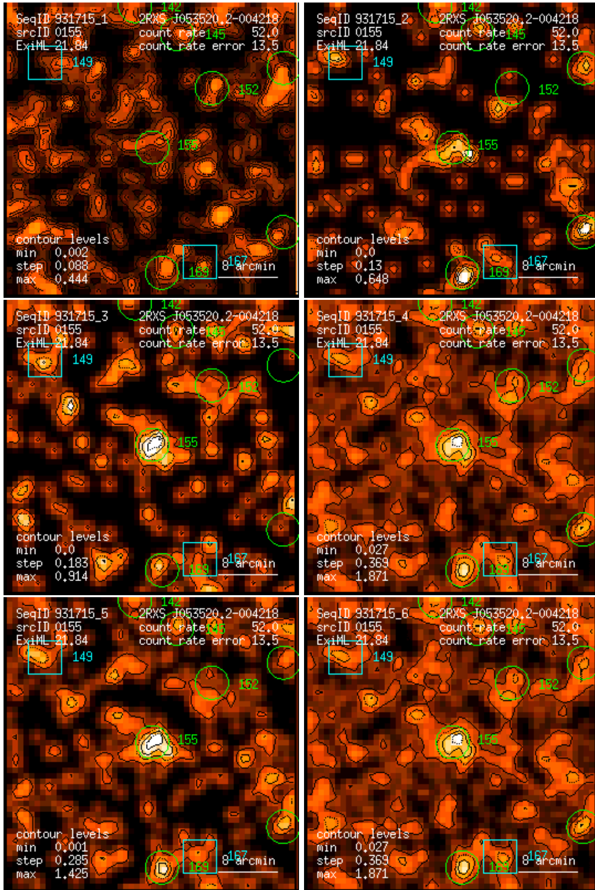
Figure 155: RASS 931715: detection 0155: band rate images, Gaussian filter: (1) PSPC channels 11 – 41, (2) 52 – 90, (3) 91 – 201, (4) 11 – 235, (5) 52 – 201, (6) 11 – 201. Broad band rates in counts/ks. Band rate contour levels in counts/ks/arcmin 2 .
