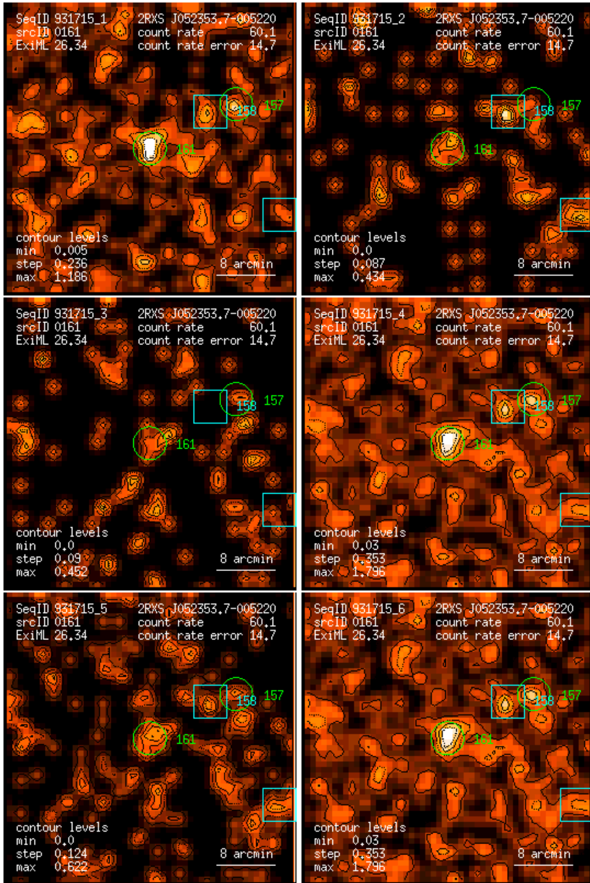
Figure 161: RASS 931715: detection 0161: band rate images, Gaussian filter: (1) PSPC channels 11 – 41, (2) 52 – 90, (3) 91 – 201, (4) 11 – 235, (5) 52 – 201, (6) 11 – 201. Broad band rates in counts/ks. Band rate contour levels in counts/ks/arcmin 2 .
