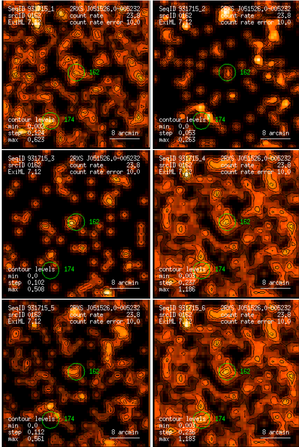
Figure 162: RASS 931715: detection 0162: band rate images, Gaussian filter: (1) PSPC channels 11 – 41, (2) 52 – 90, (3) 91 – 201, (4) 11 – 235, (5) 52 – 201, (6) 11 – 201. Broad band rates in counts/ks. Band rate contour levels in counts/ks/arcmin 2 .
