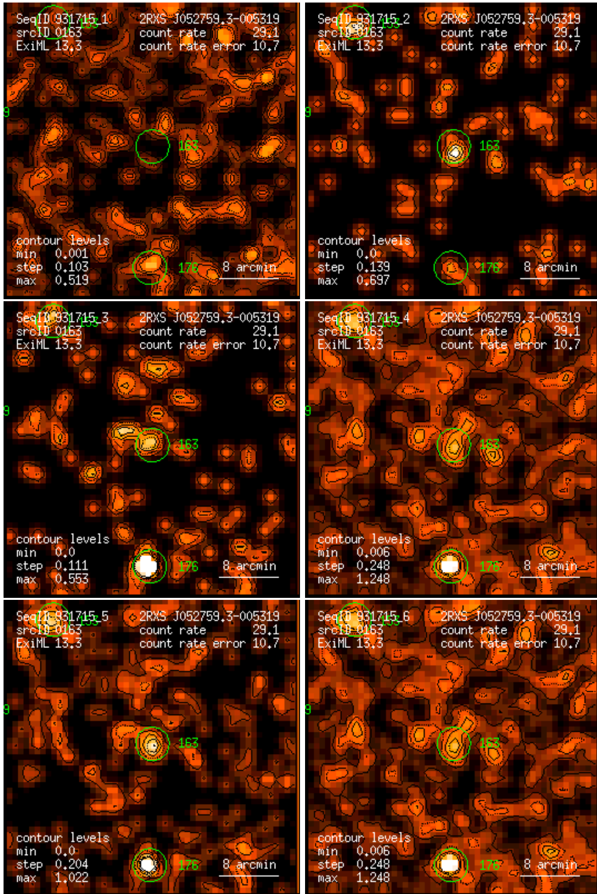
Figure 163: RASS 931715: detection 0163: band rate images, Gaussian filter: (1) PSPC channels 11 – 41, (2) 52 – 90, (3) 91 – 201, (4) 11 – 235, (5) 52 – 201, (6) 11 – 201. Broad band rates in counts/ks. Band rate contour levels in counts/ks/arcmin 2 .
