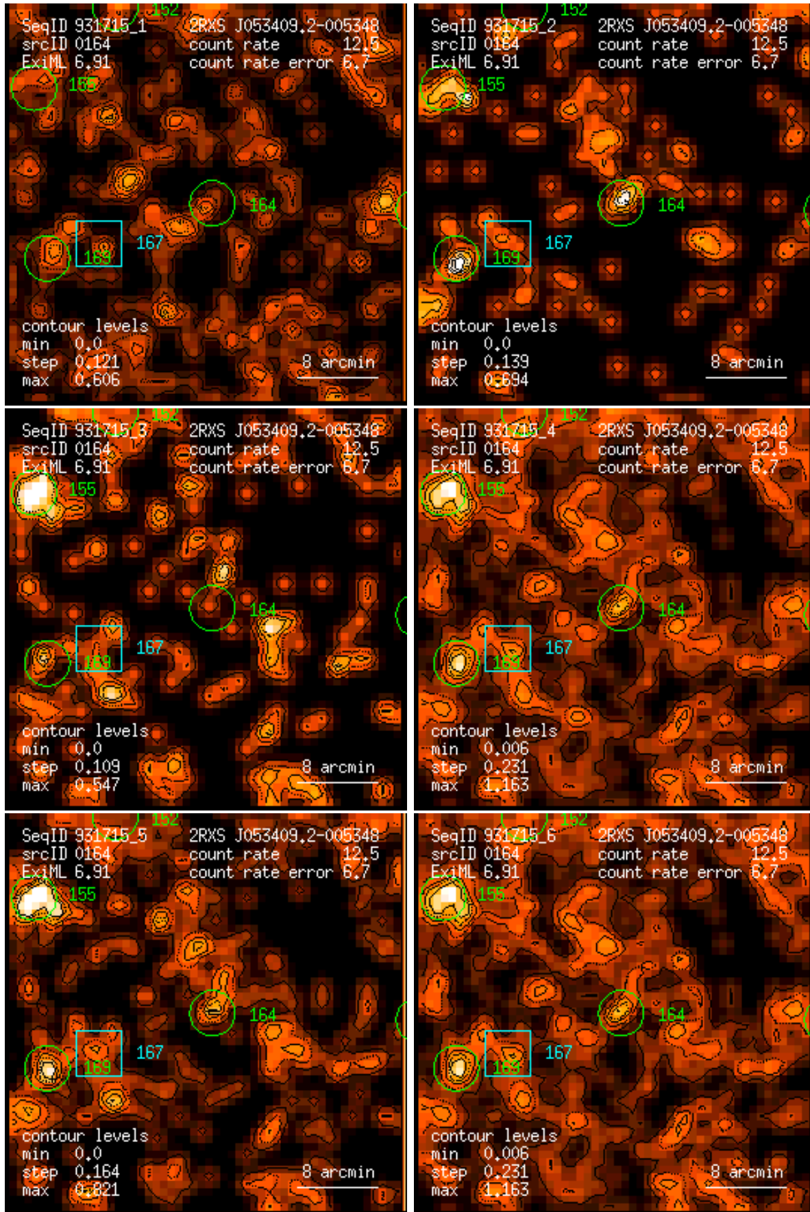
Figure 164: RASS 931715: detection 0164: band rate images, Gaussian filter: (1) PSPC channels 11 – 41, (2) 52 – 90, (3) 91 – 201, (4) 11 – 235, (5) 52 – 201, (6) 11 – 201. Broad band rates in counts/ks. Band rate contour levels in counts/ks/arcmin 2 .
