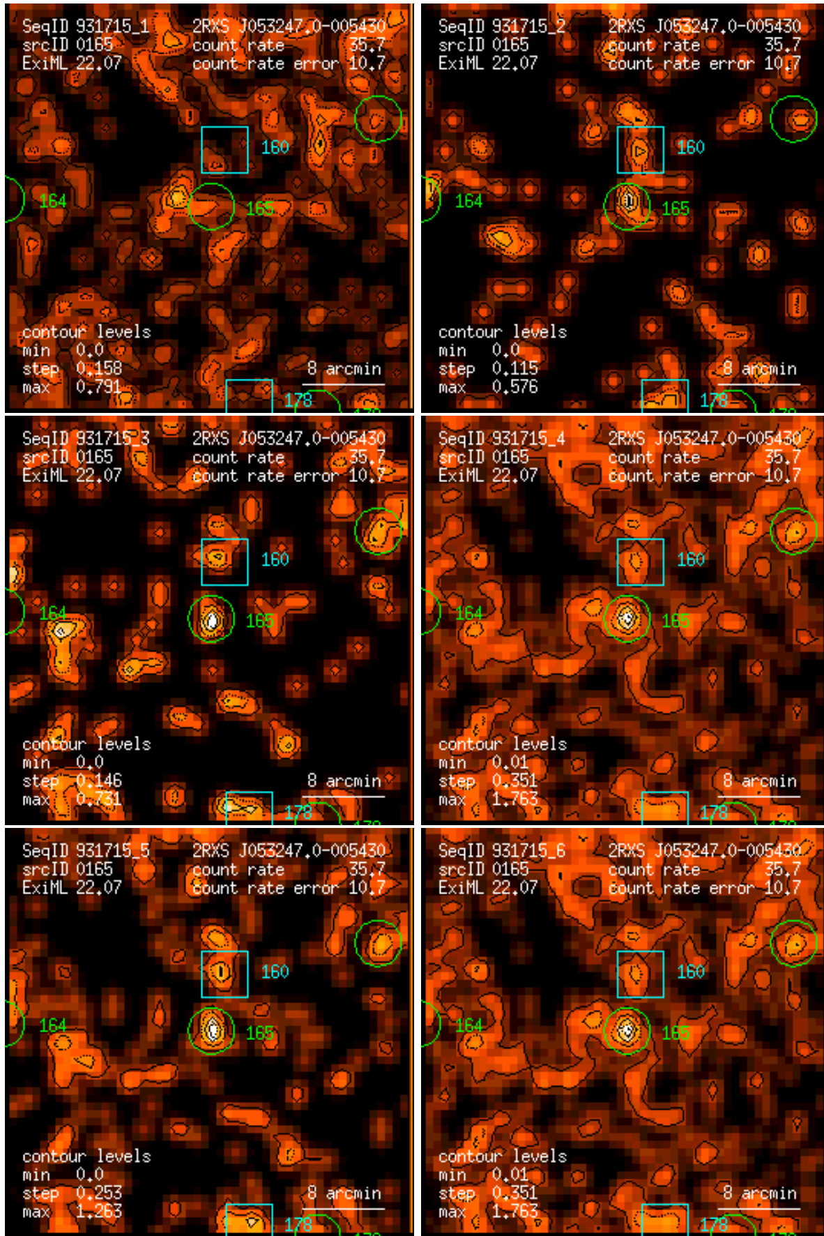
Figure 165: RASS 931715: detection 0165: band rate images, Gaussian filter: (1) PSPC channels 11 – 41, (2) 52 – 90, (3) 91 – 201, (4) 11 – 235, (5) 52 – 201, (6) 11 – 201. Broad band rates in counts/ks. Band rate contour levels in counts/ks/arcmin 2 .
