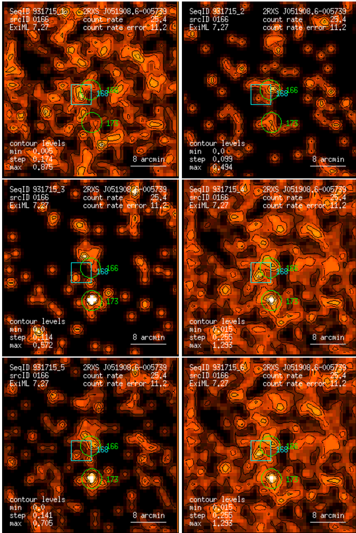
Figure 166: RASS 931715: detection 0166: band rate images, Gaussian filter: (1) PSPC channels 11 – 41, (2) 52 – 90, (3) 91 – 201, (4) 11 – 235, (5) 52 – 201, (6) 11 – 201. Broad band rates in counts/ks. Band rate contour levels in counts/ks/arcmin 2 .
