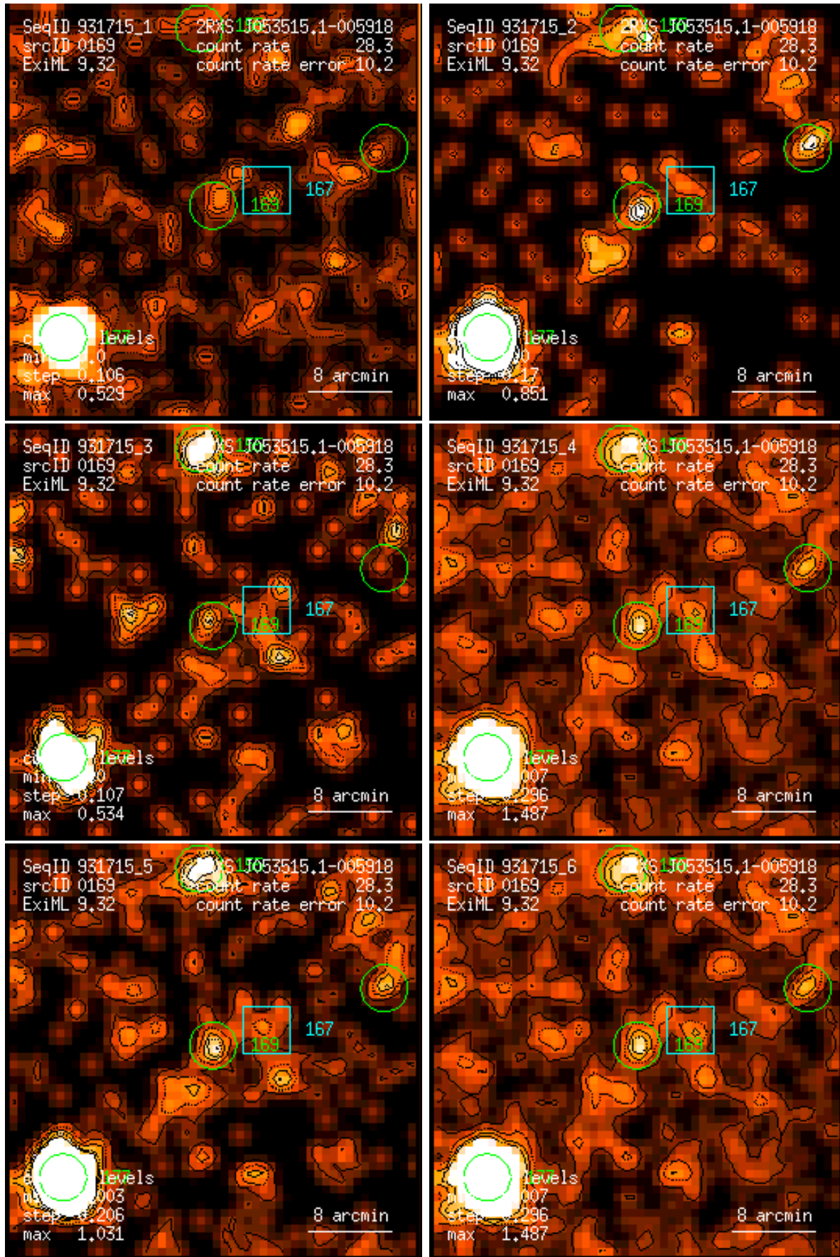
Figure 169: RASS 931715: detection 0169: band rate images, Gaussian filter: (1) PSPC channels 11 – 41, (2) 52 – 90, (3) 91 – 201, (4) 11 – 235, (5) 52 – 201, (6) 11 – 201. Broad band rates in counts/ks. Band rate contour levels in counts/ks/arcmin 2 .
