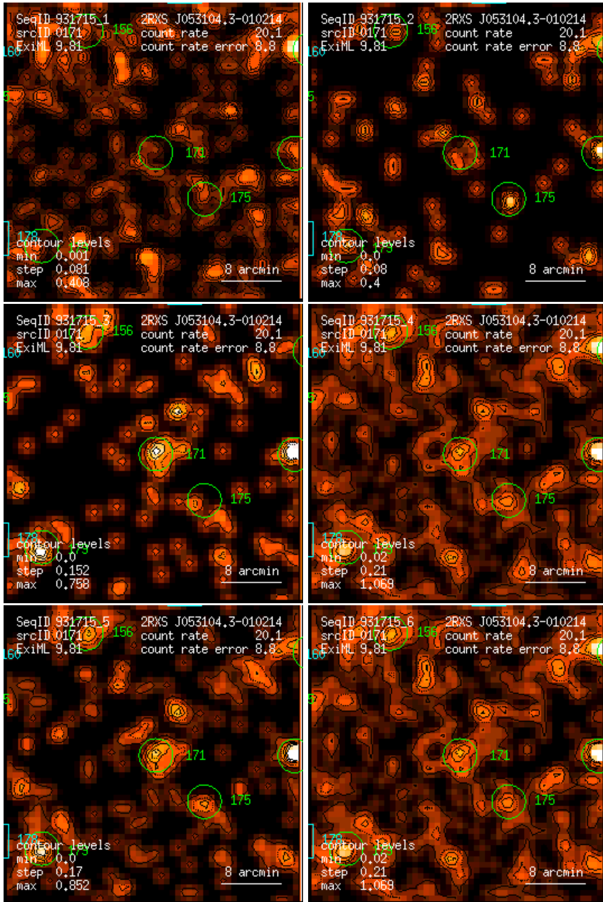
Figure 171: RASS 931715: detection 0171: band rate images, Gaussian filter: (1) PSPC channels 11 – 41, (2) 52 – 90, (3) 91 – 201, (4) 11 – 235, (5) 52 – 201, (6) 11 – 201. Broad band rates in counts/ks. Band rate contour levels in counts/ks/arcmin 2 .
