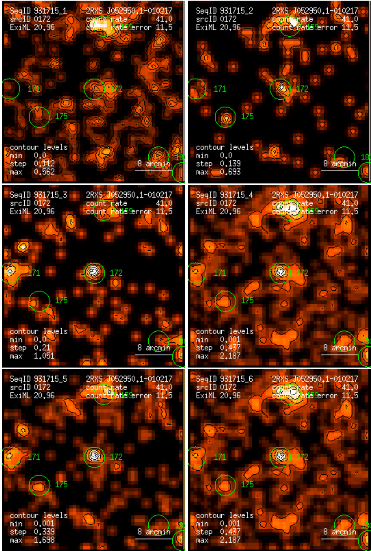
Figure 172: RASS 931715: detection 0172: band rate images, Gaussian filter: (1) PSPC channels 11 – 41, (2) 52 – 90, (3) 91 – 201, (4) 11 – 235, (5) 52 – 201, (6) 11 – 201. Broad band rates in counts/ks. Band rate contour levels in counts/ks/arcmin 2 .
