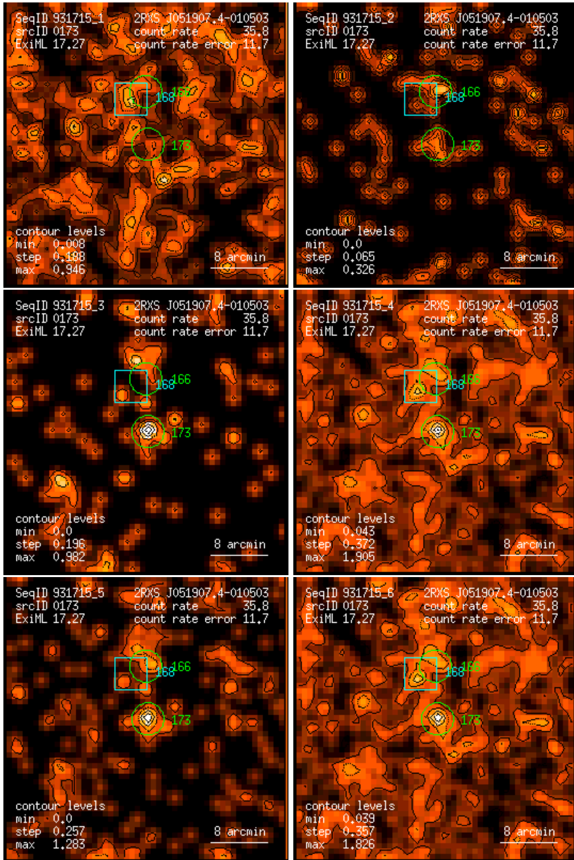
Figure 173: RASS 931715: detection 0173: band rate images, Gaussian filter: (1) PSPC channels 11 – 41, (2) 52 – 90, (3) 91 – 201, (4) 11 – 235, (5) 52 – 201, (6) 11 – 201. Broad band rates in counts/ks. Band rate contour levels in counts/ks/arcmin 2 .
