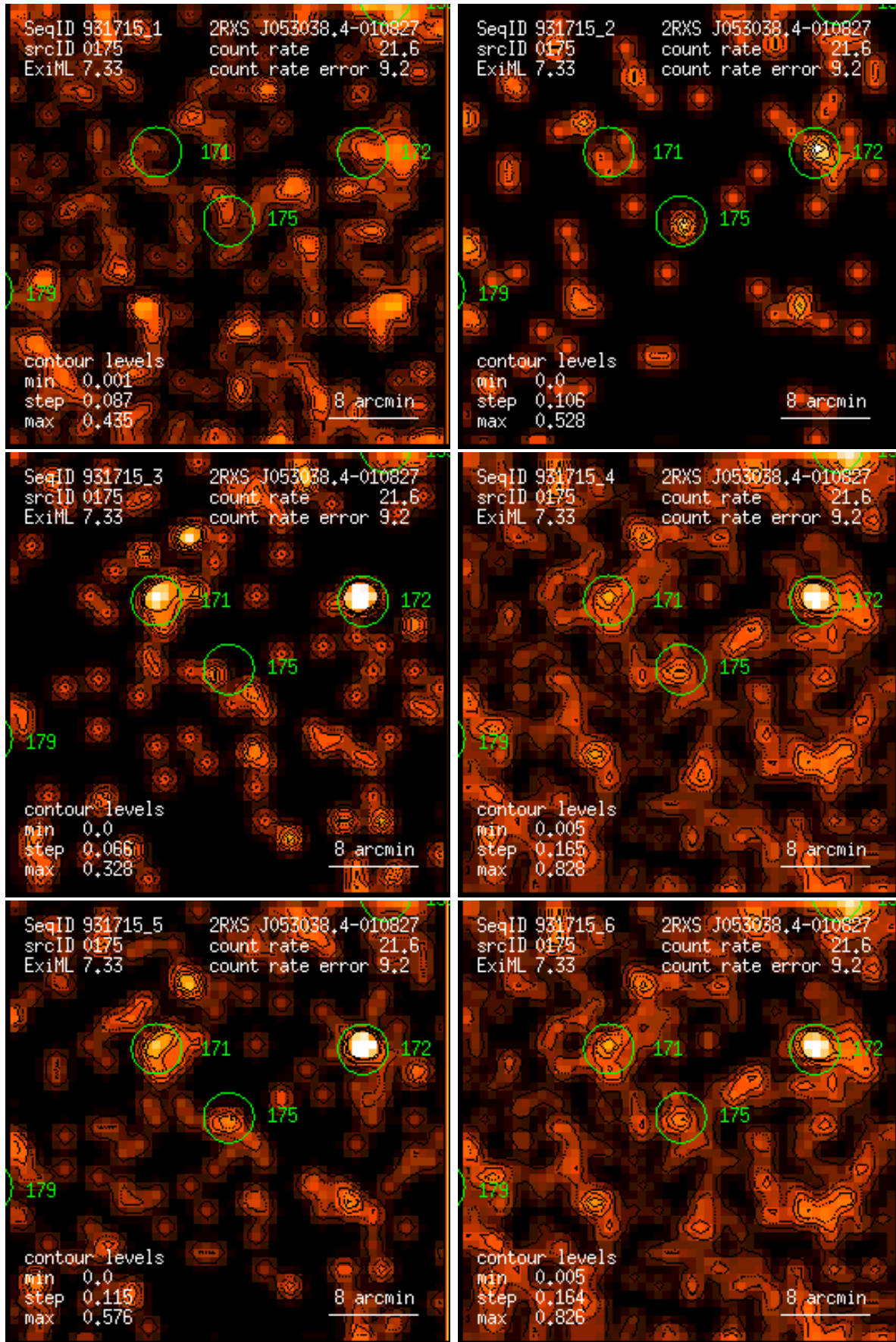
Figure 175: RASS 931715: detection 0175: band rate images, Gaussian filter: (1) PSPC channels 11 – 41, (2) 52 – 90, (3) 91 – 201, (4) 11 – 235, (5) 52 – 201, (6) 11 – 201. Broad band rates in counts/ks. Band rate contour levels in counts/ks/arcmin 2 .
