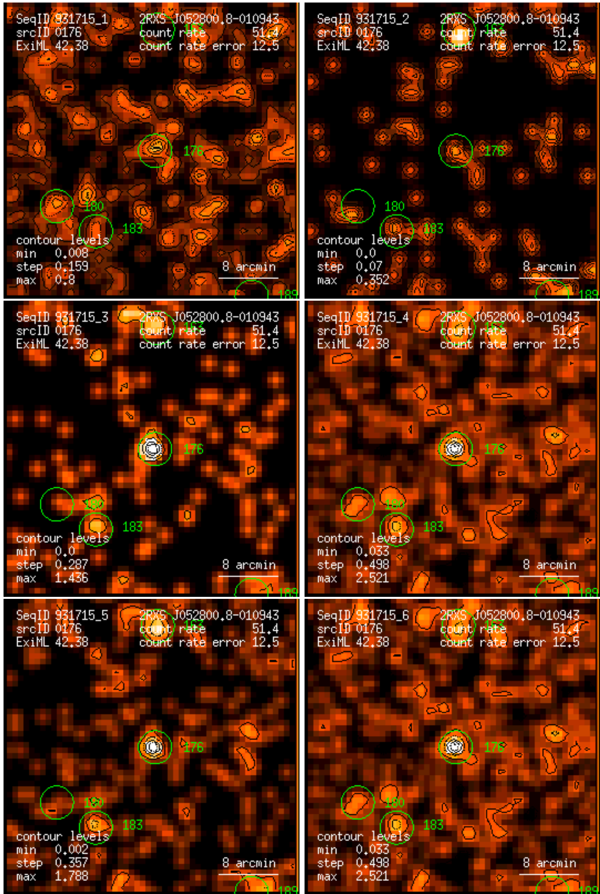
Figure 176: RASS 931715: detection 0176: band rate images, Gaussian filter: (1) PSPC channels 11 – 41, (2) 52 – 90, (3) 91 – 201, (4) 11 – 235, (5) 52 – 201, (6) 11 – 201. Broad band rates in counts/ks. Band rate contour levels in counts/ks/arcmin 2 .
