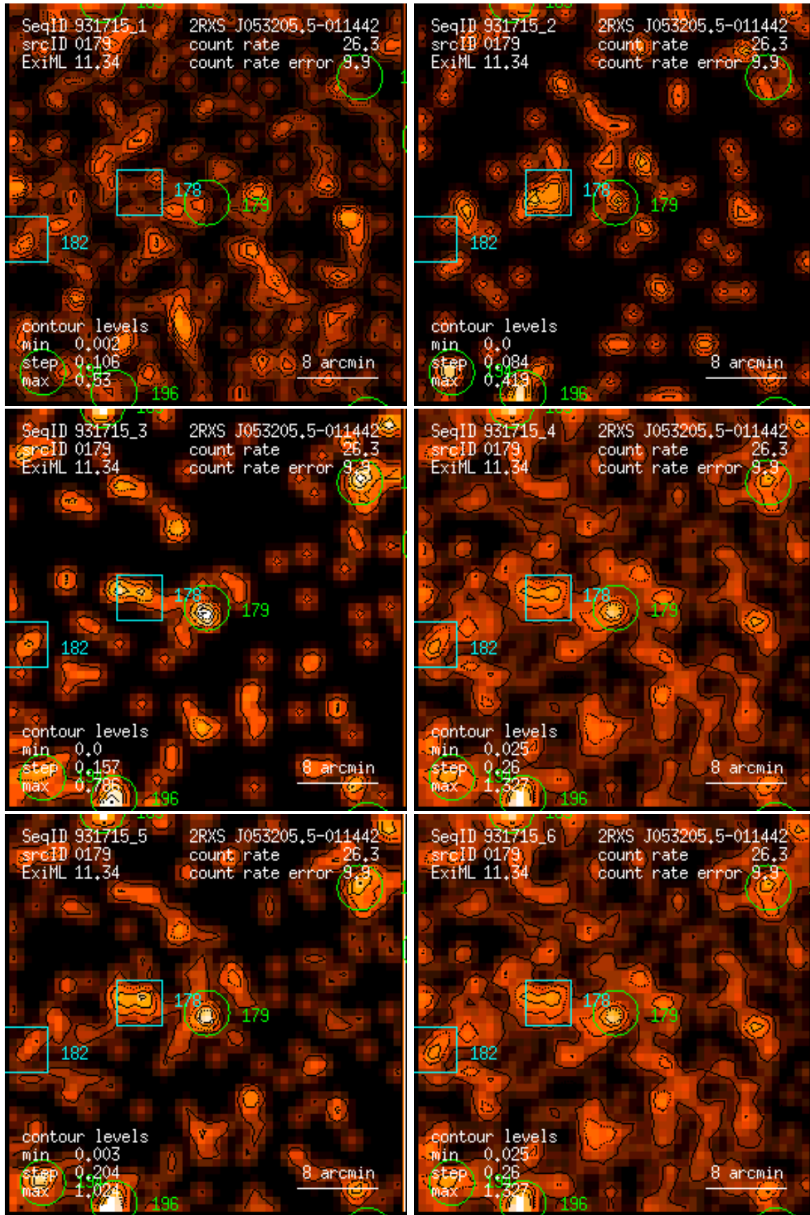
Figure 179: RASS 931715: detection 0179: band rate images, Gaussian filter: (1) PSPC channels 11 – 41, (2) 52 – 90, (3) 91 – 201, (4) 11 – 235, (5) 52 – 201, (6) 11 – 201. Broad band rates in counts/ks. Band rate contour levels in counts/ks/arcmin 2 .
