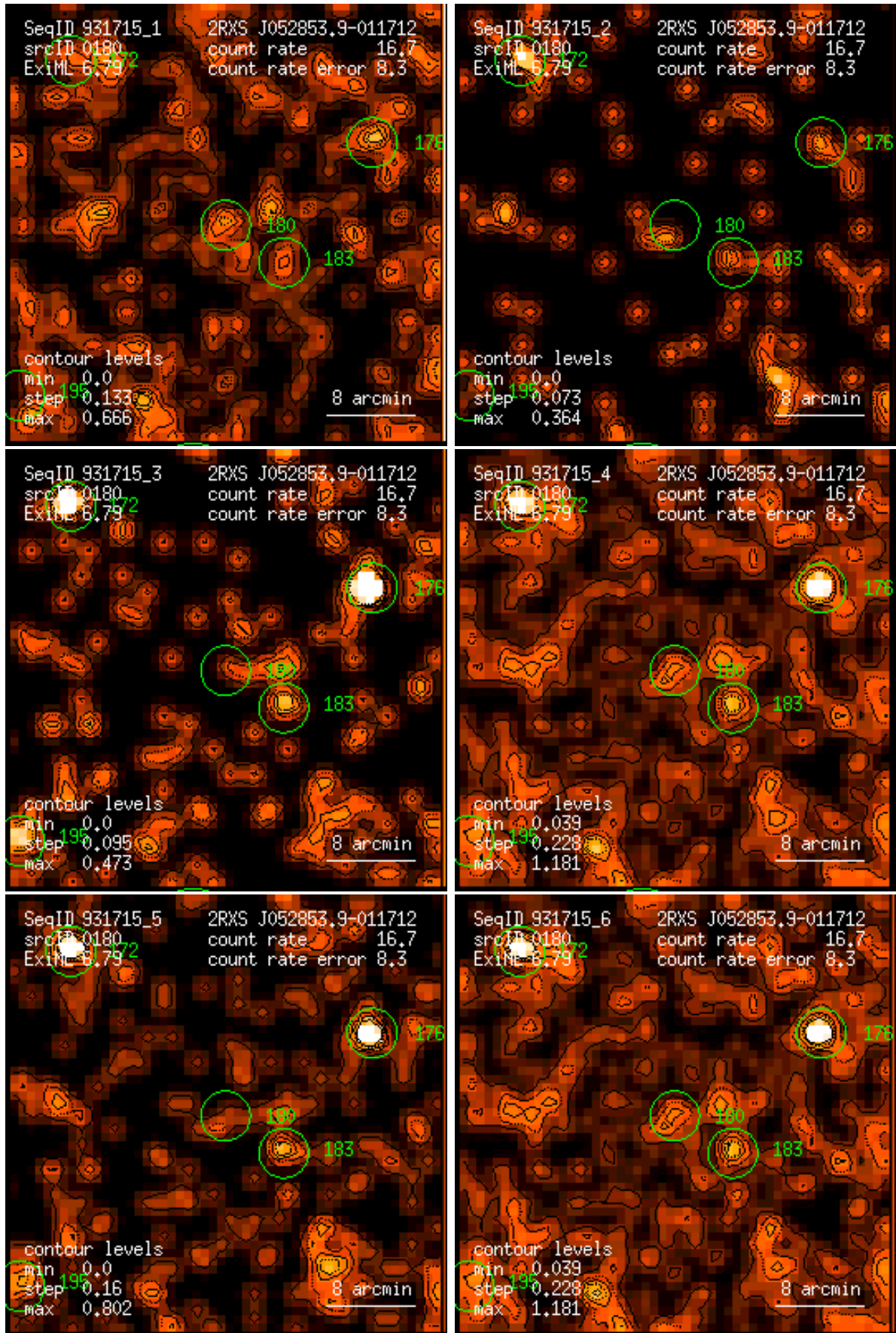
Figure 180: RASS 931715: detection 0180: band rate images, Gaussian filter: (1) PSPC channels 11 – 41, (2) 52 – 90, (3) 91 – 201, (4) 11 – 235, (5) 52 – 201, (6) 11 – 201. Broad band rates in counts/ks. Band rate contour levels in counts/ks/arcmin 2 .
