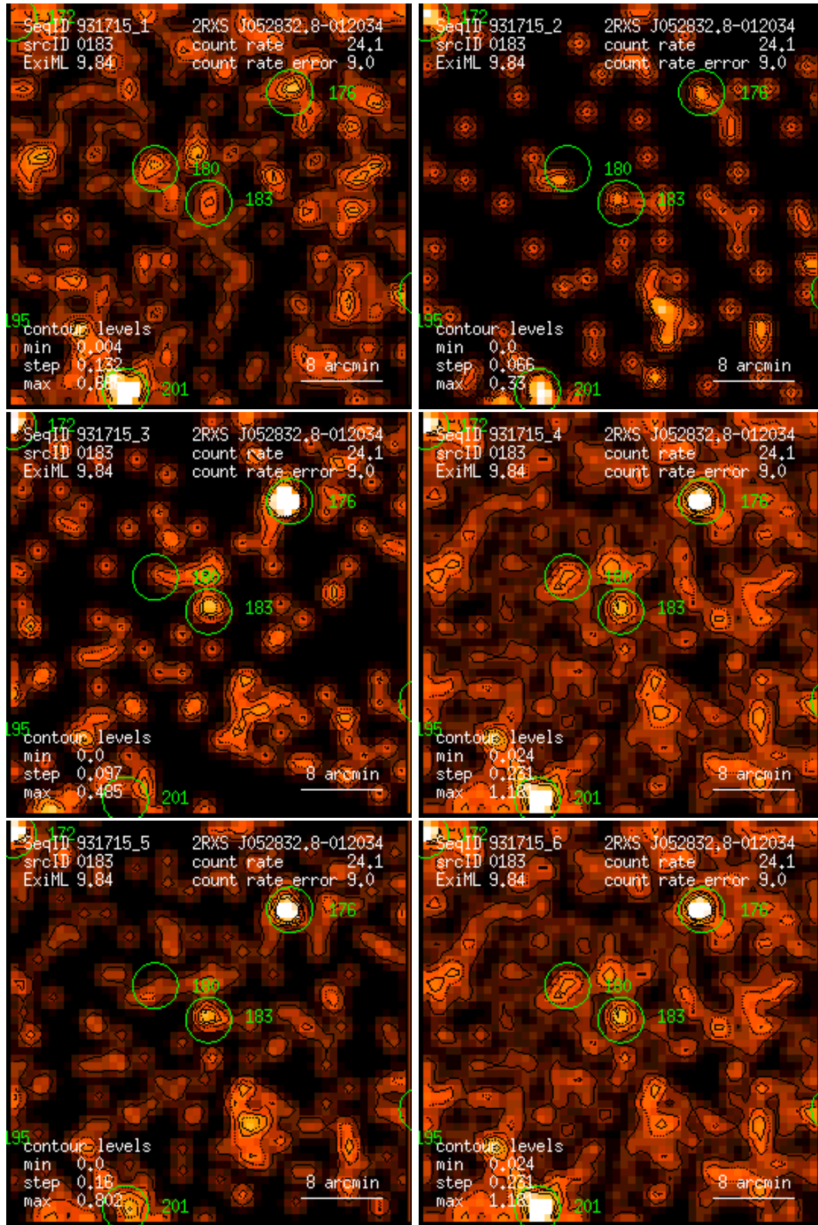
Figure 183: RASS 931715: detection 0183: band rate images, Gaussian filter: (1) PSPC channels 11 – 41, (2) 52 – 90, (3) 91 – 201, (4) 11 – 235, (5) 52 – 201, (6) 11 – 201. Broad band rates in counts/ks. Band rate contour levels in counts/ks/arcmin 2 .
