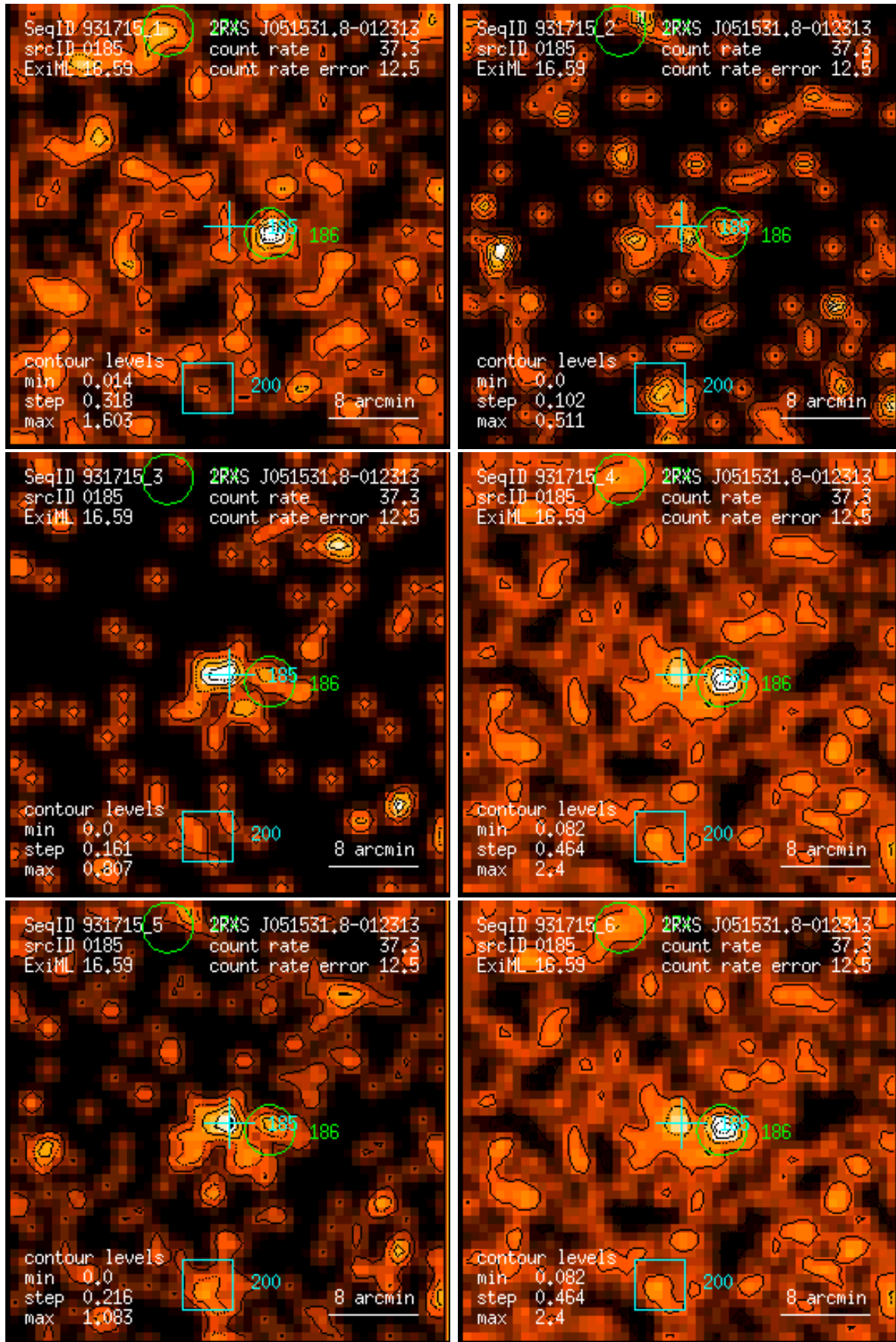
Figure 185: RASS 931715: detection 0185: band rate images, Gaussian filter: (1) PSPC channels 11 – 41, (2) 52 – 90, (3) 91 – 201, (4) 11 – 235, (5) 52 – 201, (6) 11 – 201. Broad band rates in counts/ks. Band rate contour levels in counts/ks/arcmin 2 .
