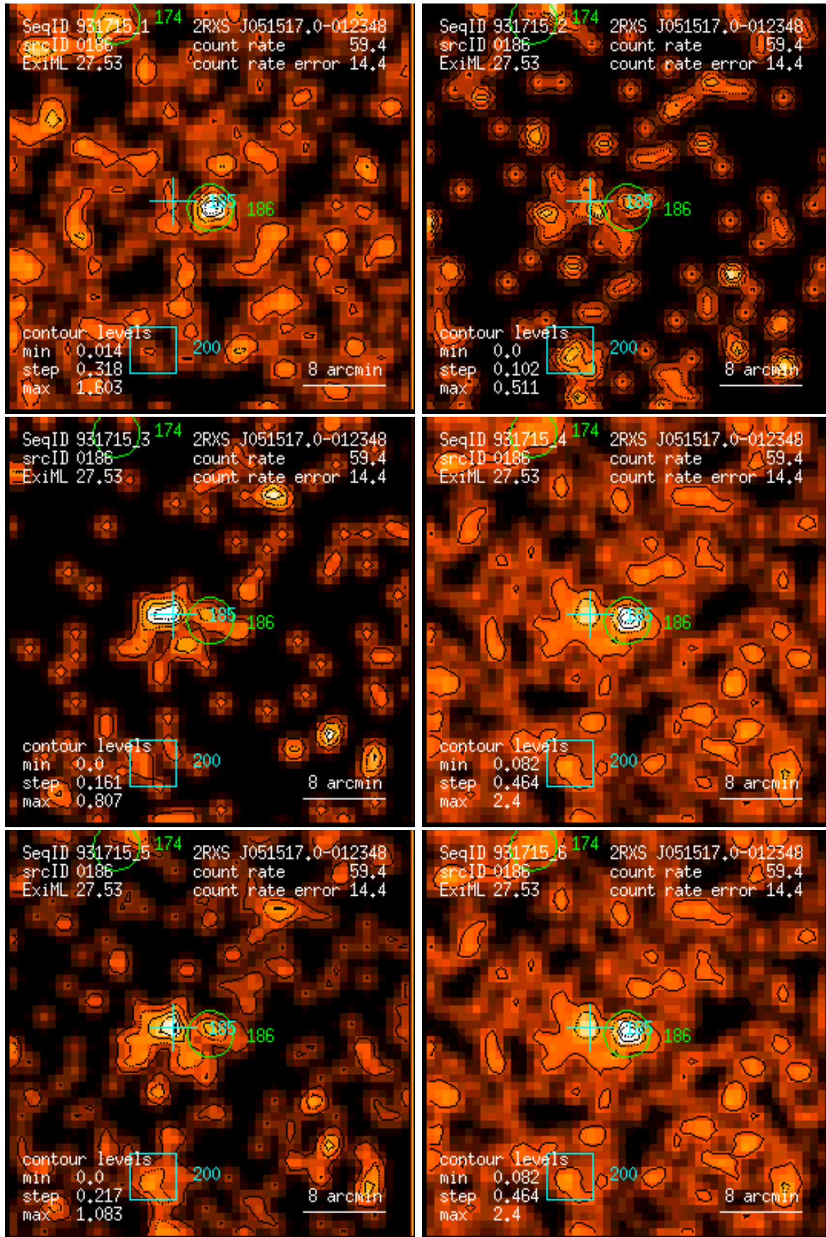
Figure 186: RASS 931715: detection 0186: band rate images, Gaussian filter: (1) PSPC channels 11 – 41, (2) 52 – 90, (3) 91 – 201, (4) 11 – 235, (5) 52 – 201, (6) 11 – 201. Broad band rates in counts/ks. Band rate contour levels in counts/ks/arcmin 2 .
