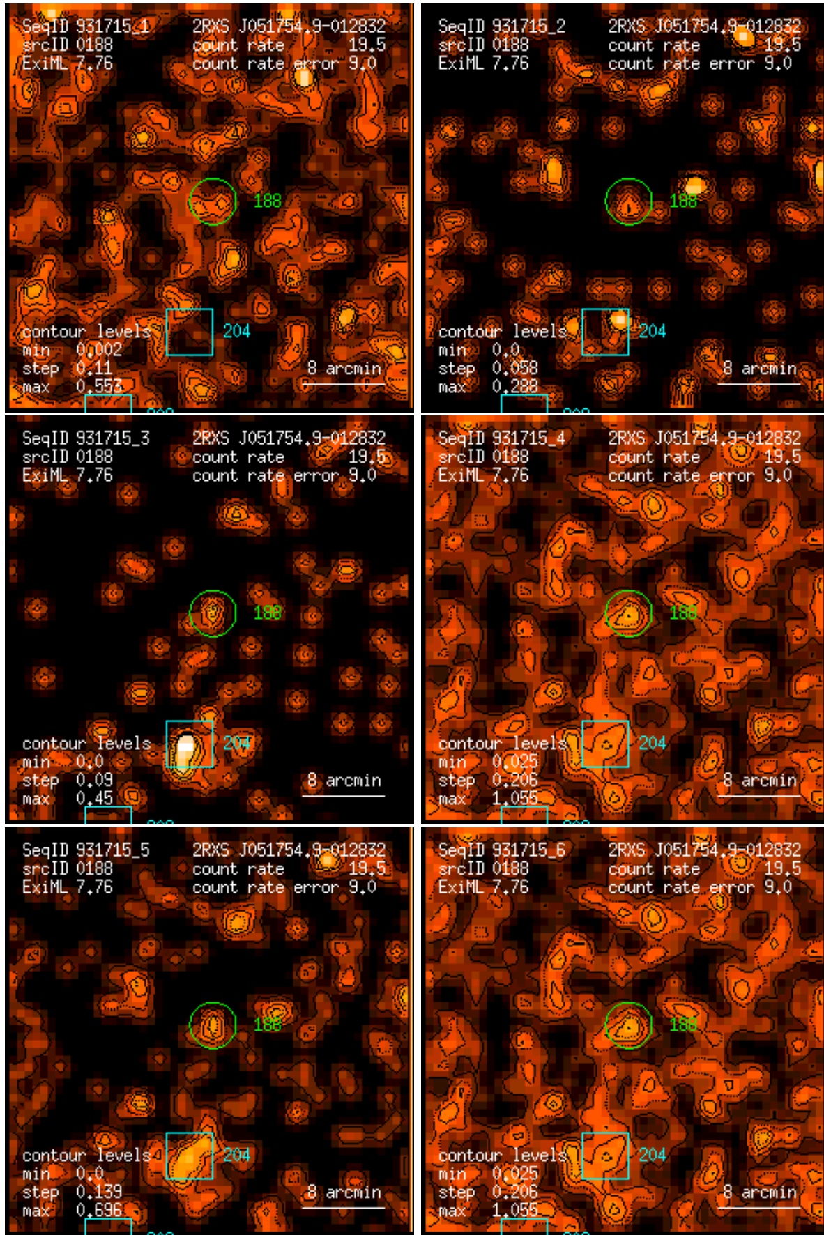
Figure 188: RASS 931715: detection 0188: band rate images, Gaussian filter: (1) PSPC channels 11 – 41, (2) 52 – 90, (3) 91 – 201, (4) 11 – 235, (5) 52 – 201, (6) 11 – 201. Broad band rates in counts/ks. Band rate contour levels in counts/ks/arcmin 2 .
