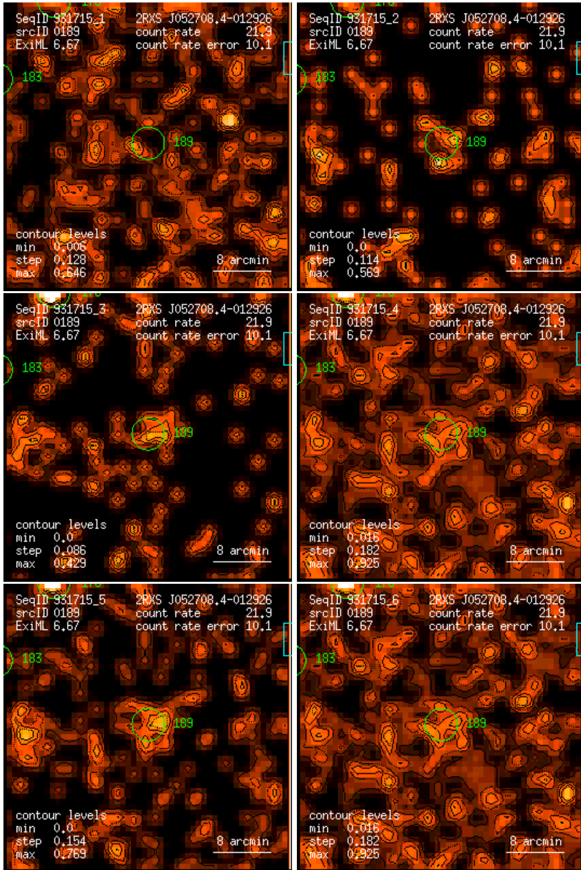
Figure 189: RASS 931715: detection 0189: band rate images, Gaussian filter: (1) PSPC channels 11 – 41, (2) 52 – 90, (3) 91 – 201, (4) 11 – 235, (5) 52 – 201, (6) 11 – 201. Broad band rates in counts/ks. Band rate contour levels in counts/ks/arcmin 2 .
