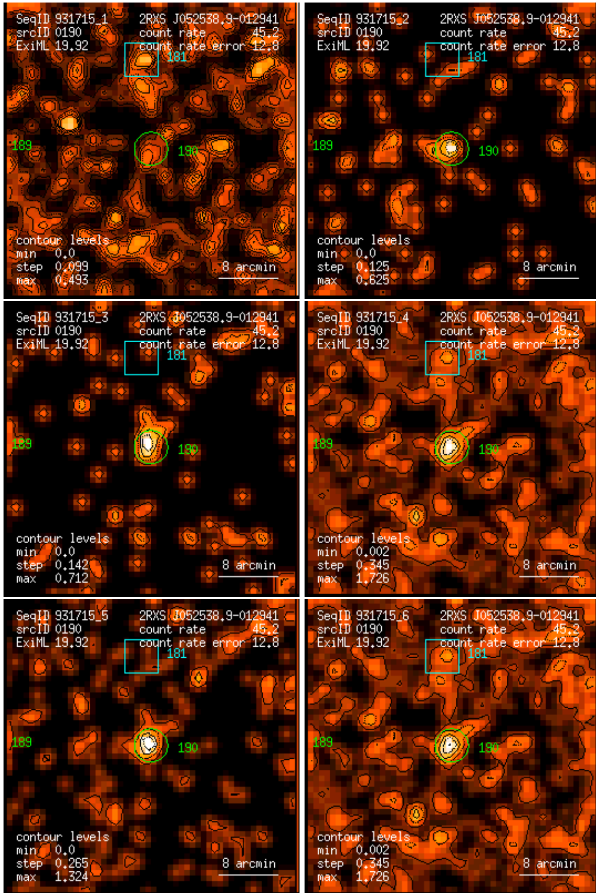
Figure 190: RASS 931715: detection 0190: band rate images, Gaussian filter: (1) PSPC channels 11 – 41, (2) 52 – 90, (3) 91 – 201, (4) 11 – 235, (5) 52 – 201, (6) 11 – 201. Broad band rates in counts/ks. Band rate contour levels in counts/ks/arcmin 2 .
