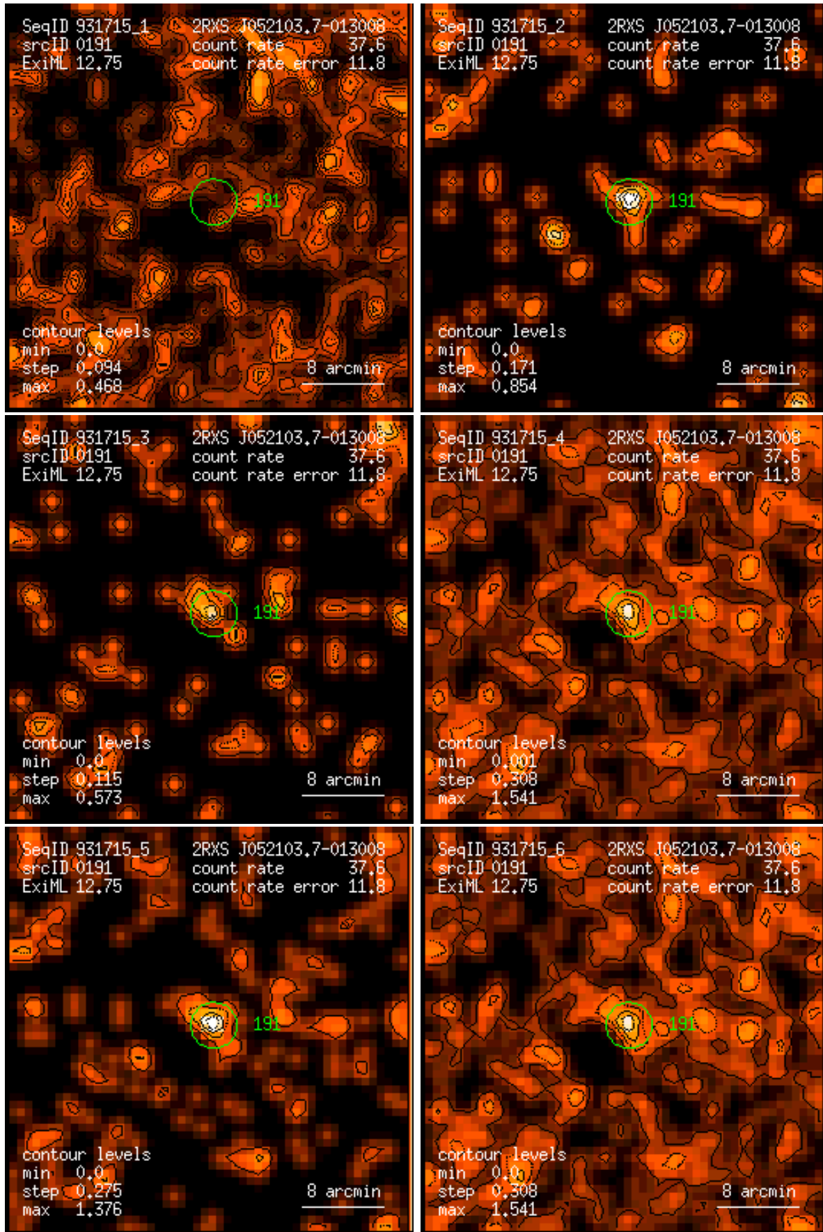
Figure 191: RASS 931715: detection 0191: band rate images, Gaussian filter: (1) PSPC channels 11 – 41, (2) 52 – 90, (3) 91 – 201, (4) 11 – 235, (5) 52 – 201, (6) 11 – 201. Broad band rates in counts/ks. Band rate contour levels in counts/ks/arcmin 2 .
