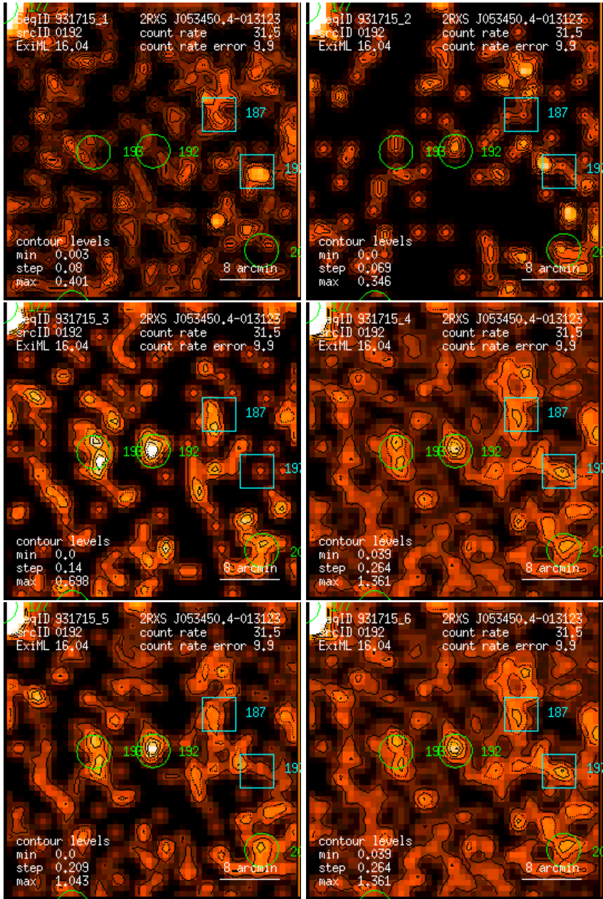
Figure 192: RASS 931715: detection 0192: band rate images, Gaussian filter: (1) PSPC channels 11 – 41, (2) 52 – 90, (3) 91 – 201, (4) 11 – 235, (5) 52 – 201, (6) 11 – 201. Broad band rates in counts/ks. Band rate contour levels in counts/ks/arcmin 2 .
