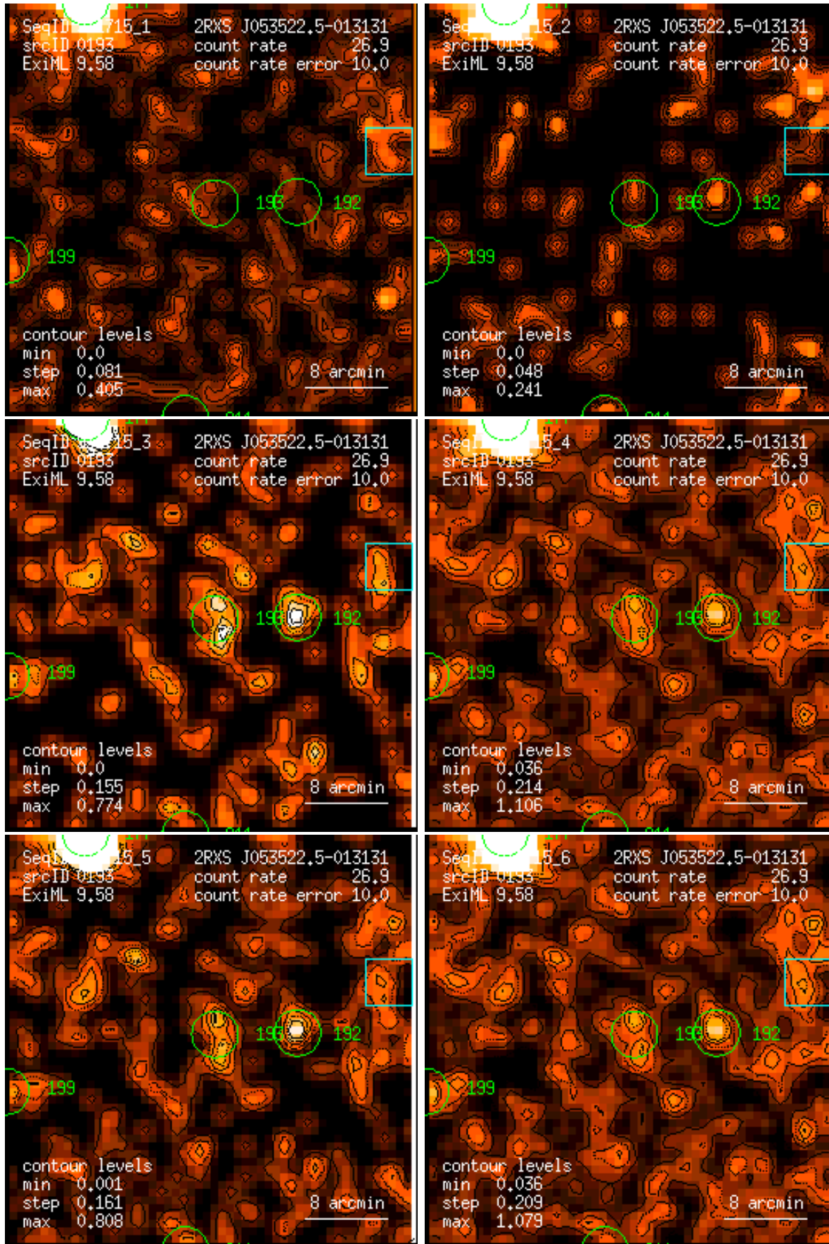
Figure 193: RASS 931715: detection 0193: band rate images, Gaussian filter: (1) PSPC channels 11 – 41, (2) 52 – 90, (3) 91 – 201, (4) 11 – 235, (5) 52 – 201, (6) 11 – 201. Broad band rates in counts/ks. Band rate contour levels in counts/ks/arcmin 2 .
