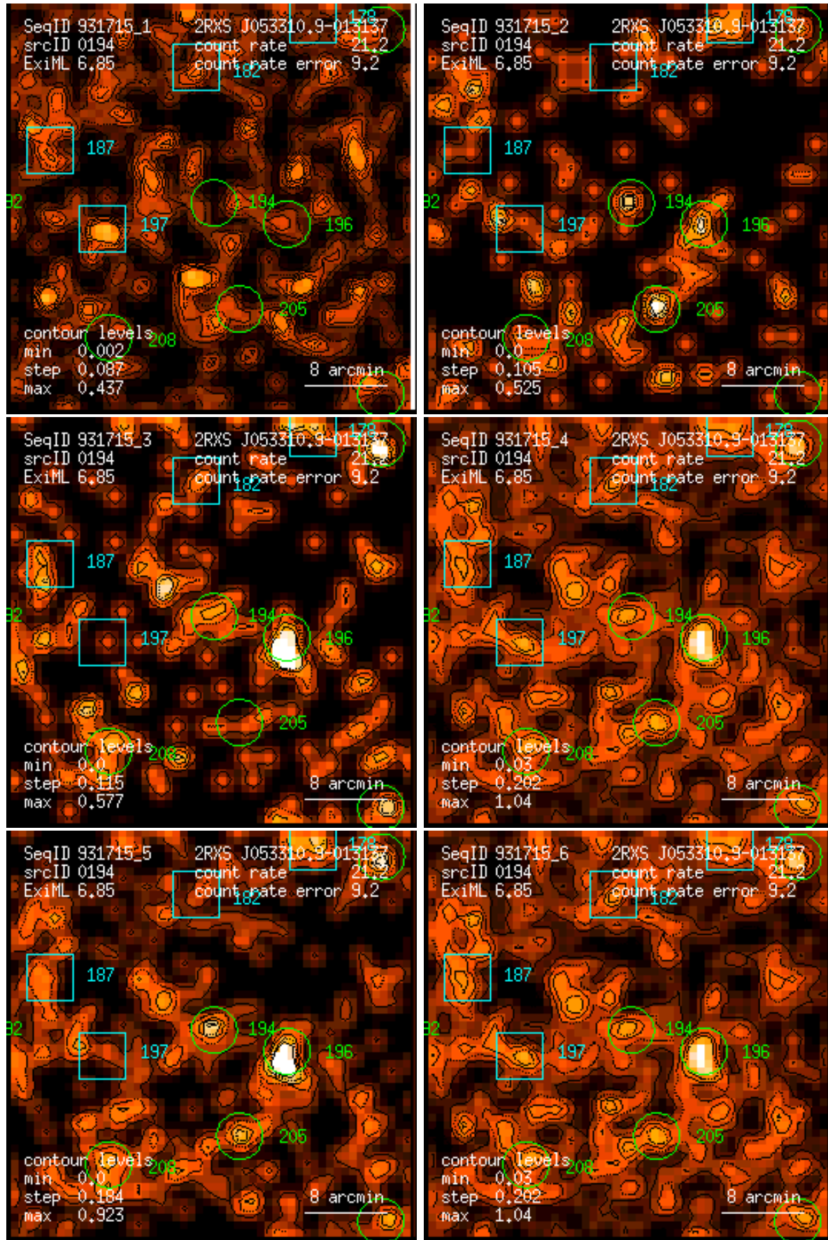
Figure 194: RASS 931715: detection 0194: band rate images, Gaussian filter: (1) PSPC channels 11 – 41, (2) 52 – 90, (3) 91 – 201, (4) 11 – 235, (5) 52 – 201, (6) 11 – 201. Broad band rates in counts/ks. Band rate contour levels in counts/ks/arcmin 2 .
