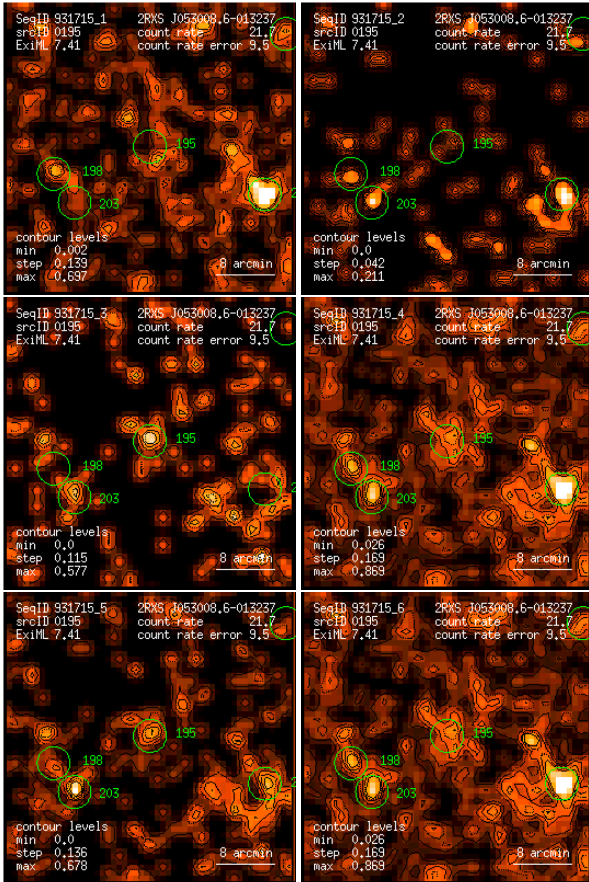
Figure 195: RASS 931715: detection 0195: band rate images, Gaussian filter: (1) PSPC channels 11 – 41, (2) 52 – 90, (3) 91 – 201, (4) 11 – 235, (5) 52 – 201, (6) 11 – 201. Broad band rates in counts/ks. Band rate contour levels in counts/ks/arcmin 2 .
