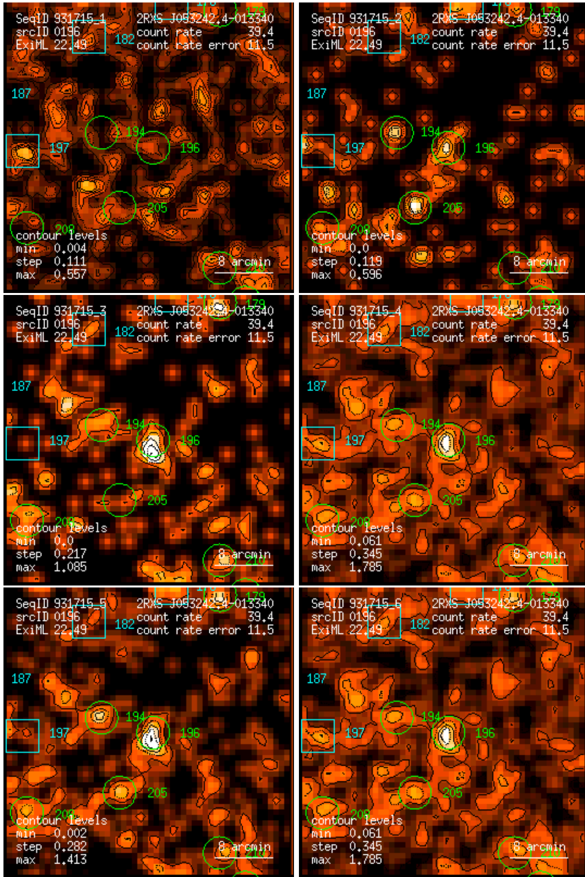
Figure 196: RASS 931715: detection 0196: band rate images, Gaussian filter: (1) PSPC channels 11 – 41, (2) 52 – 90, (3) 91 – 201, (4) 11 – 235, (5) 52 – 201, (6) 11 – 201. Broad band rates in counts/ks. Band rate contour levels in counts/ks/arcmin 2 .
