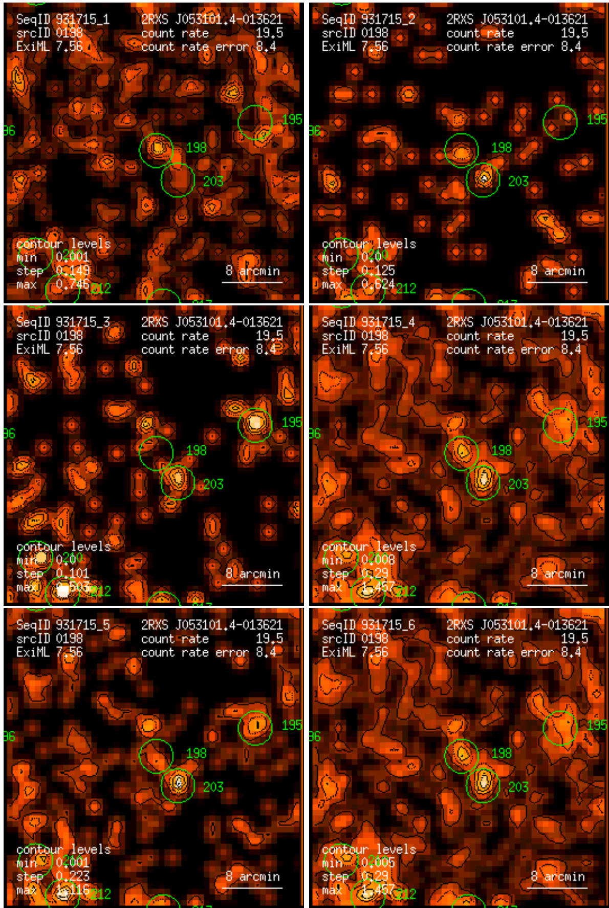
Figure 198: RASS 931715: detection 0198: band rate images, Gaussian filter: (1) PSPC channels 11 – 41, (2) 52 – 90, (3) 91 – 201, (4) 11 – 235, (5) 52 – 201, (6) 11 – 201. Broad band rates in counts/ks. Band rate contour levels in counts/ks/arcmin 2 .
