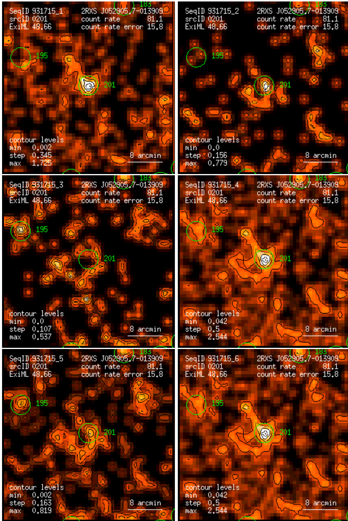
Figure 201: RASS 931715: detection 0201: band rate images, Gaussian filter: (1) PSPC channels 11 – 41, (2) 52 – 90, (3) 91 – 201, (4) 11 – 235, (5) 52 – 201, (6) 11 – 201. Broad band rates in counts/ks. Band rate contour levels in counts/ks/arcmin 2 .
