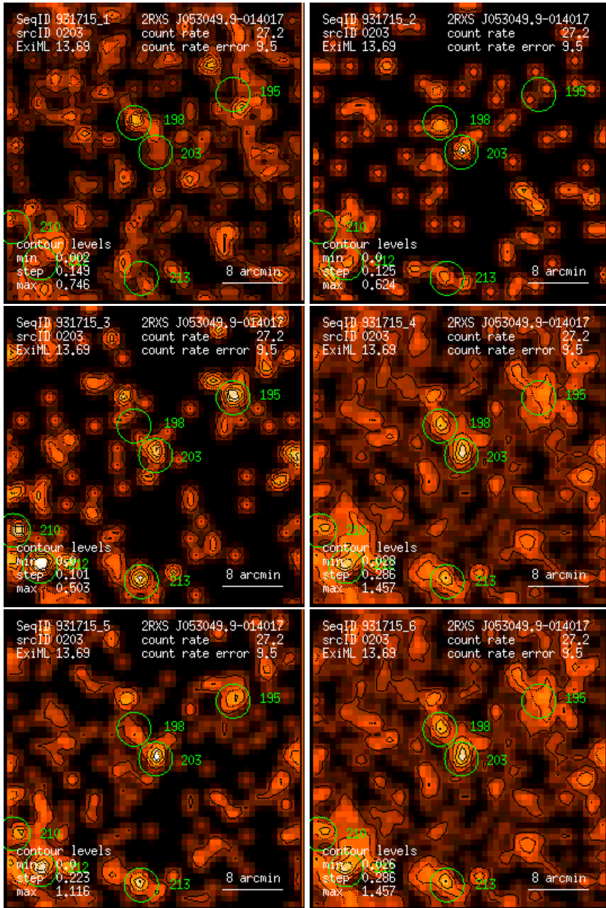
Figure 203: RASS 931715: detection 0203: band rate images, Gaussian filter: (1) PSPC channels 11 – 41, (2) 52 – 90, (3) 91 – 201, (4) 11 – 235, (5) 52 – 201, (6) 11 – 201. Broad band rates in counts/ks. Band rate contour levels in counts/ks/arcmin 2 .
