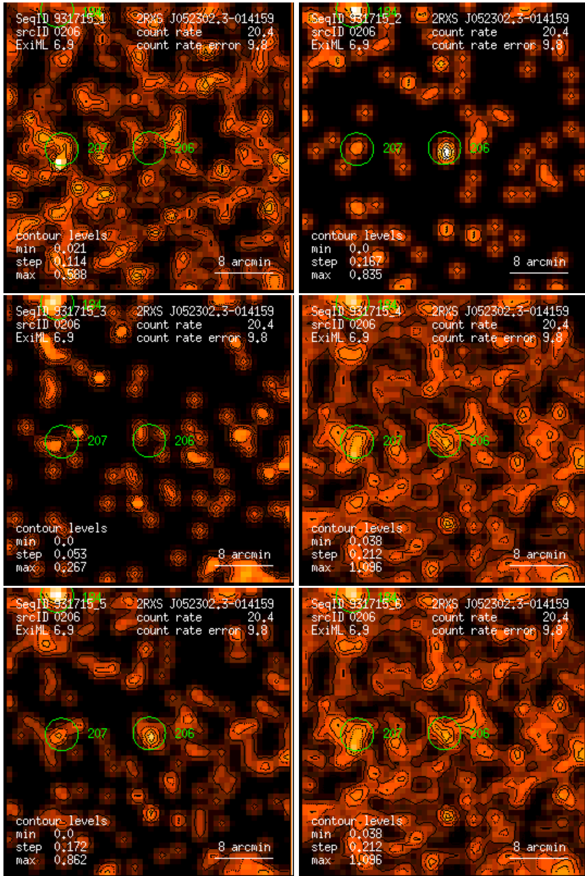
Figure 206: RASS 931715: detection 0206: band rate images, Gaussian filter: (1) PSPC channels 11 – 41, (2) 52 – 90, (3) 91 – 201, (4) 11 – 235, (5) 52 – 201, (6) 11 – 201. Broad band rates in counts/ks. Band rate contour levels in counts/ks/arcmin 2 .
