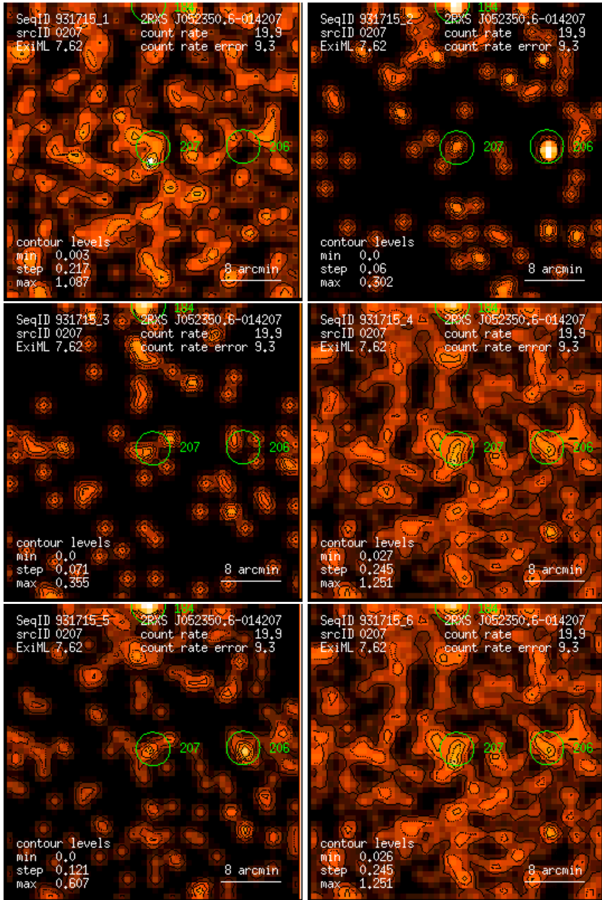
Figure 207: RASS 931715: detection 0207: band rate images, Gaussian filter: (1) PSPC channels 11 – 41, (2) 52 – 90, (3) 91 – 201, (4) 11 – 235, (5) 52 – 201, (6) 11 – 201. Broad band rates in counts/ks. Band rate contour levels in counts/ks/arcmin 2 .
