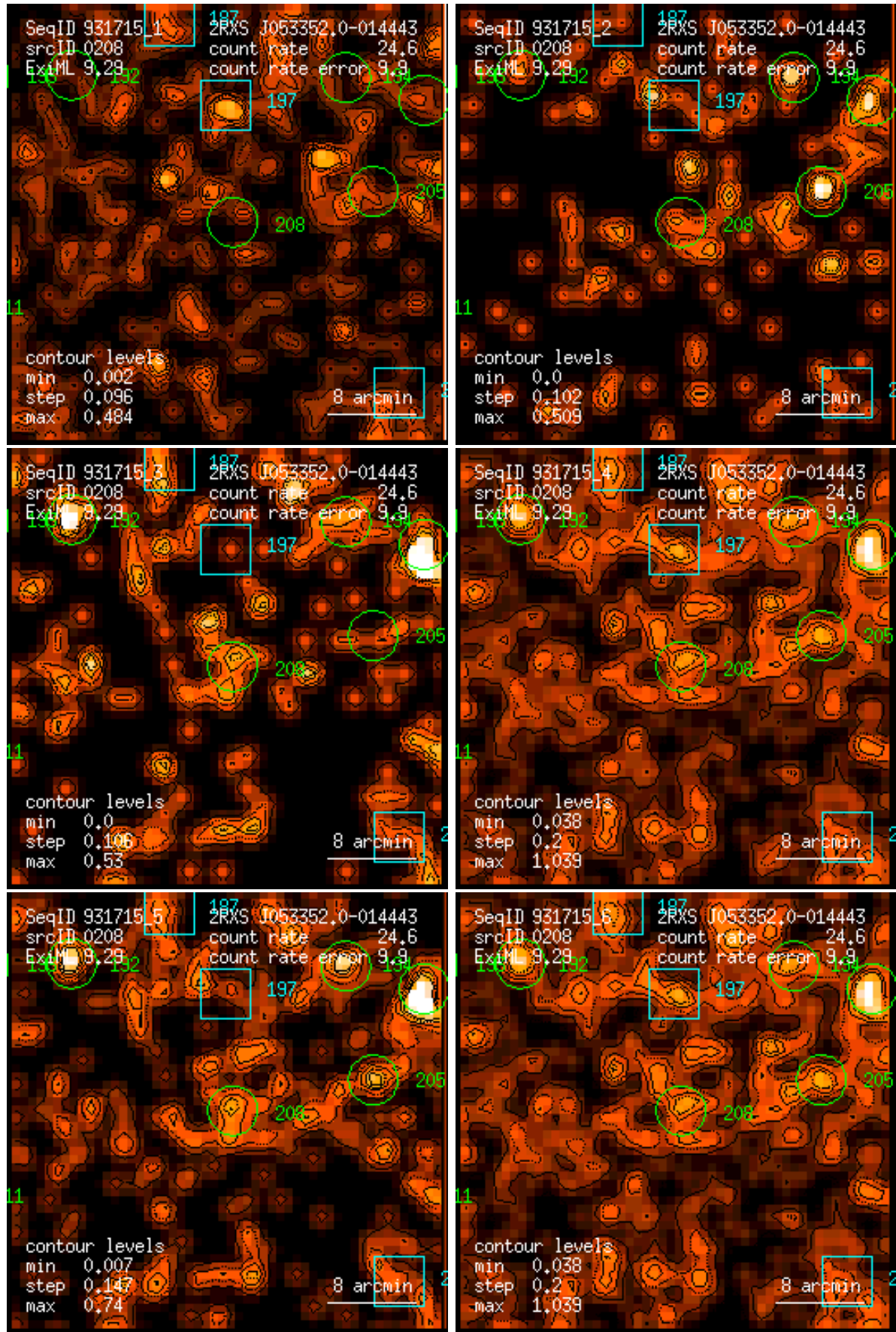
Figure 208: RASS 931715: detection 0208: band rate images, Gaussian filter: (1) PSPC channels 11 – 41, (2) 52 – 90, (3) 91 – 201, (4) 11 – 235, (5) 52 – 201, (6) 11 – 201. Broad band rates in counts/ks. Band rate contour levels in counts/ks/arcmin 2 .
