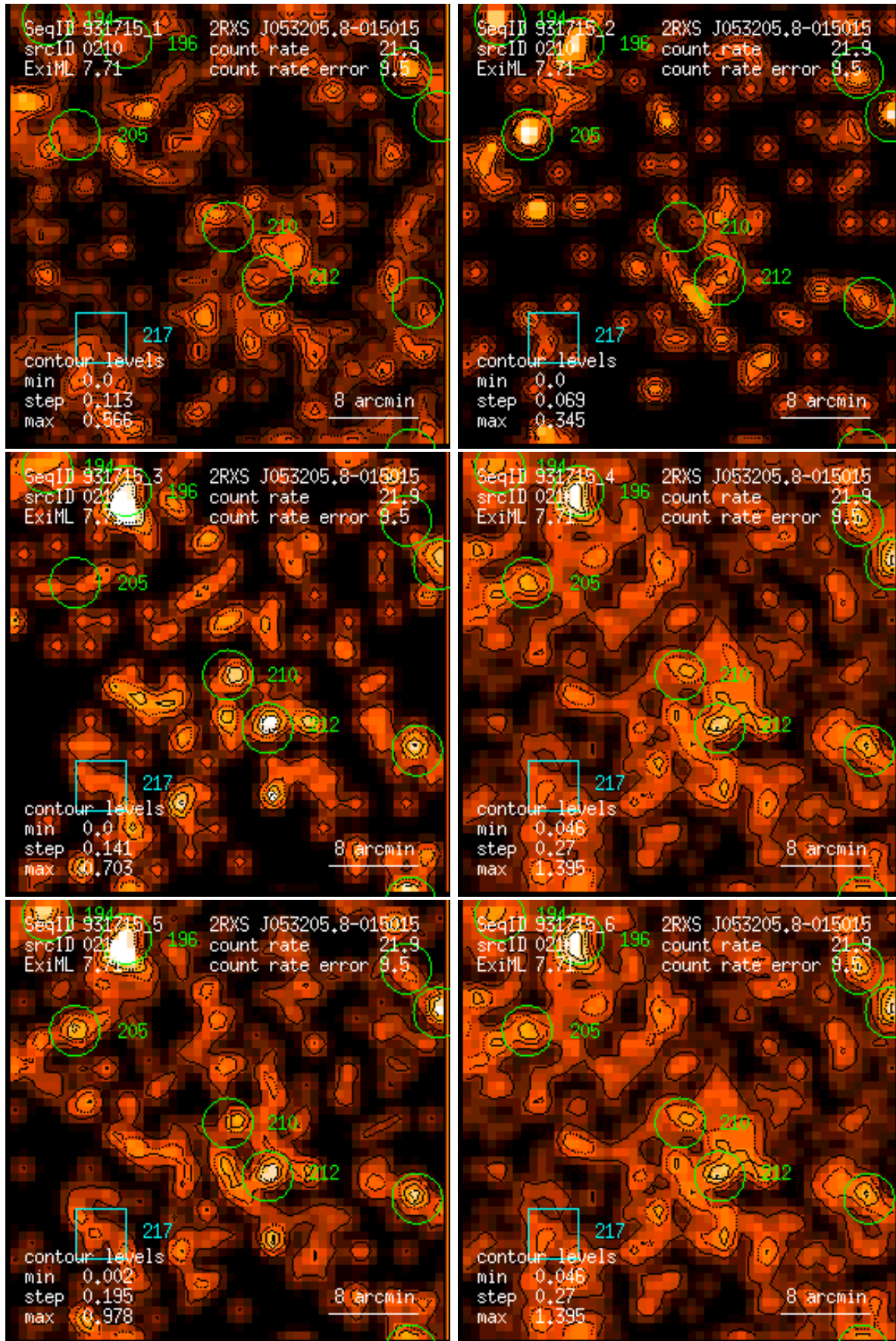
Figure 210: RASS 931715: detection 0210: band rate images, Gaussian filter: (1) PSPC channels 11 – 41, (2) 52 – 90, (3) 91 – 201, (4) 11 – 235, (5) 52 – 201, (6) 11 – 201. Broad band rates in counts/ks. Band rate contour levels in counts/ks/arcmin 2 .
