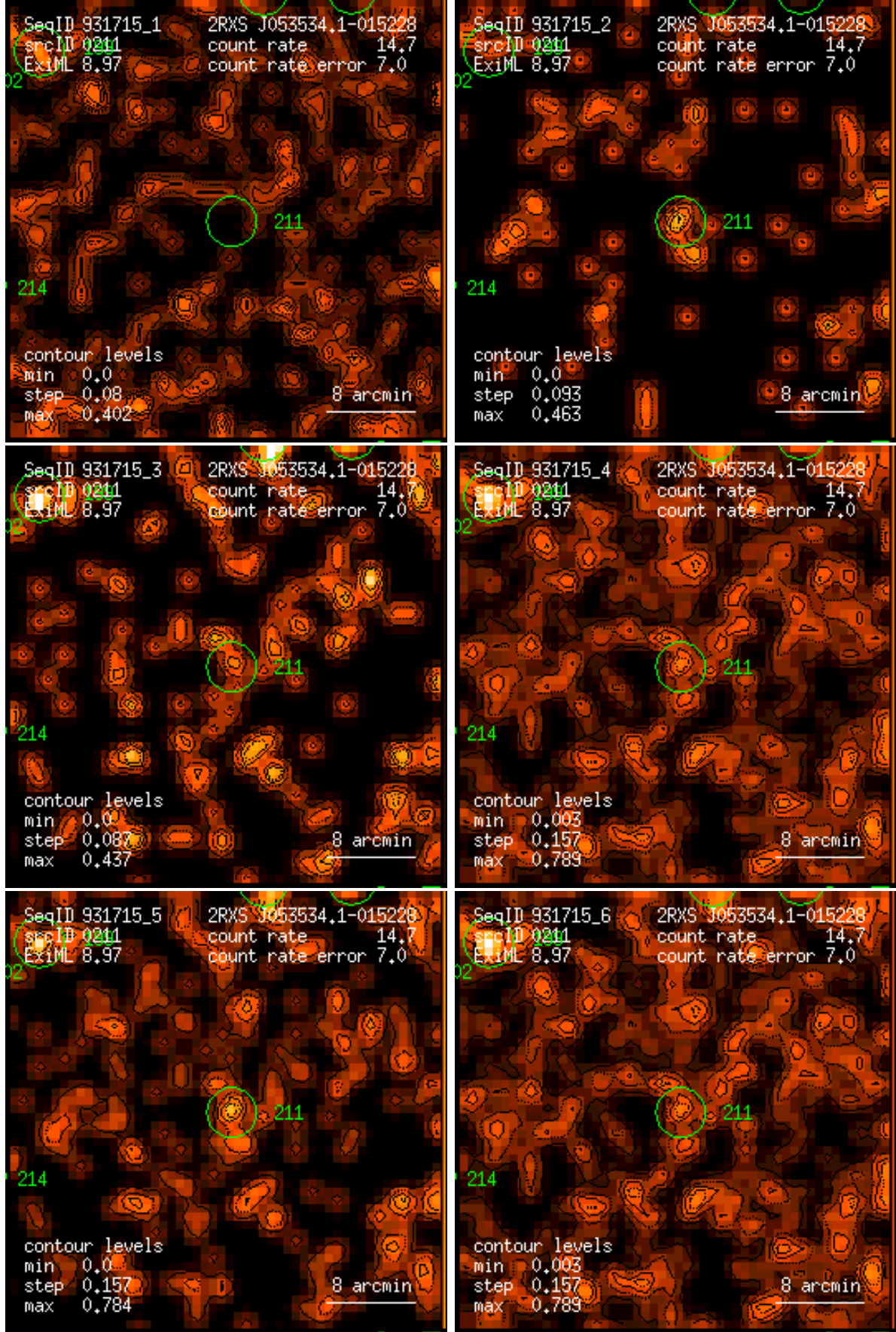
Figure 211: RASS 931715: detection 0211: band rate images, Gaussian filter: (1) PSPC channels 11 – 41, (2) 52 – 90, (3) 91 – 201, (4) 11 – 235, (5) 52 – 201, (6) 11 – 201. Broad band rates in counts/ks. Band rate contour levels in counts/ks/arcmin 2 .
