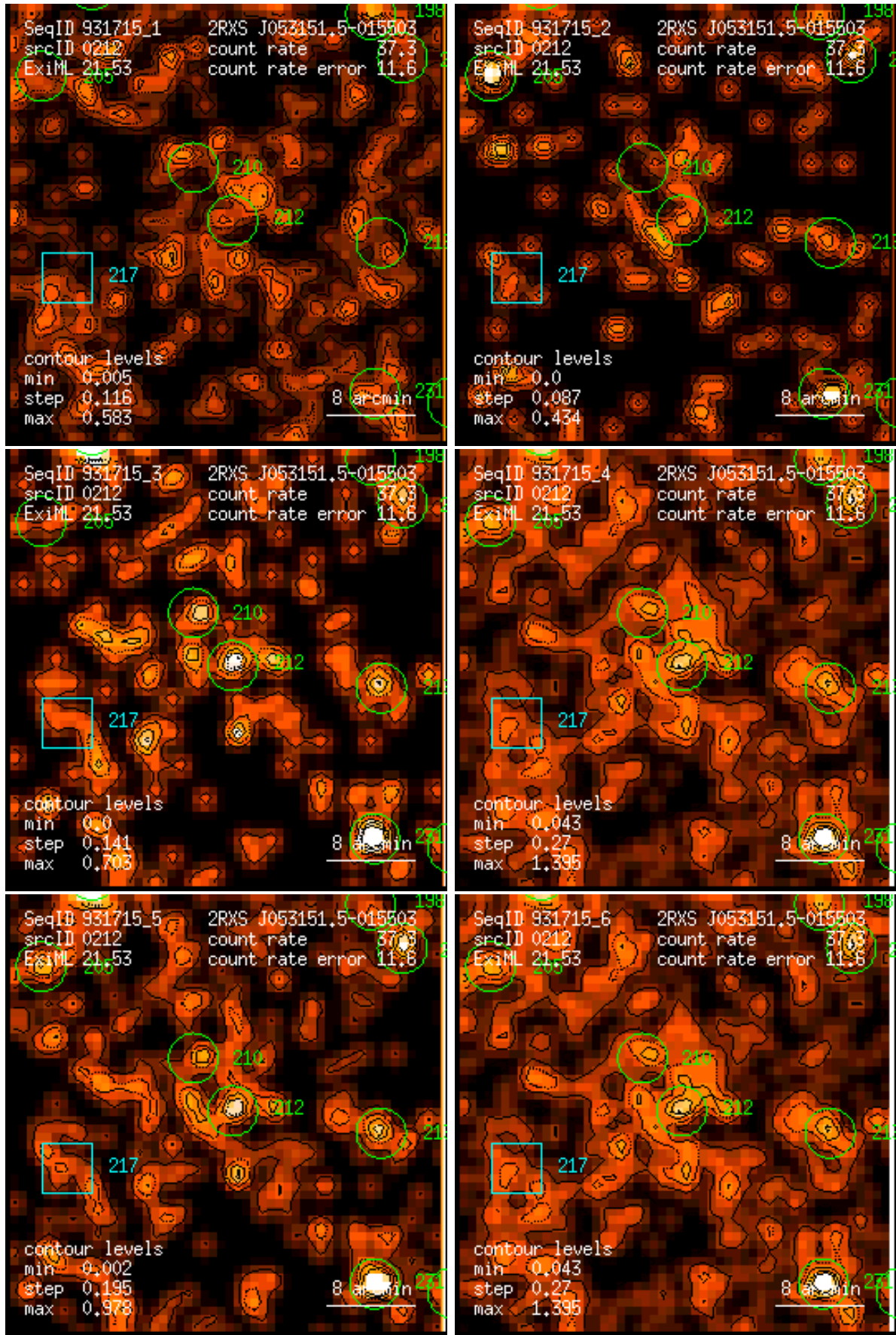
Figure 212: RASS 931715: detection 0212: band rate images, Gaussian filter: (1) PSPC channels 11 – 41, (2) 52 – 90, (3) 91 – 201, (4) 11 – 235, (5) 52 – 201, (6) 11 – 201. Broad band rates in counts/ks. Band rate contour levels in counts/ks/arcmin 2 .
