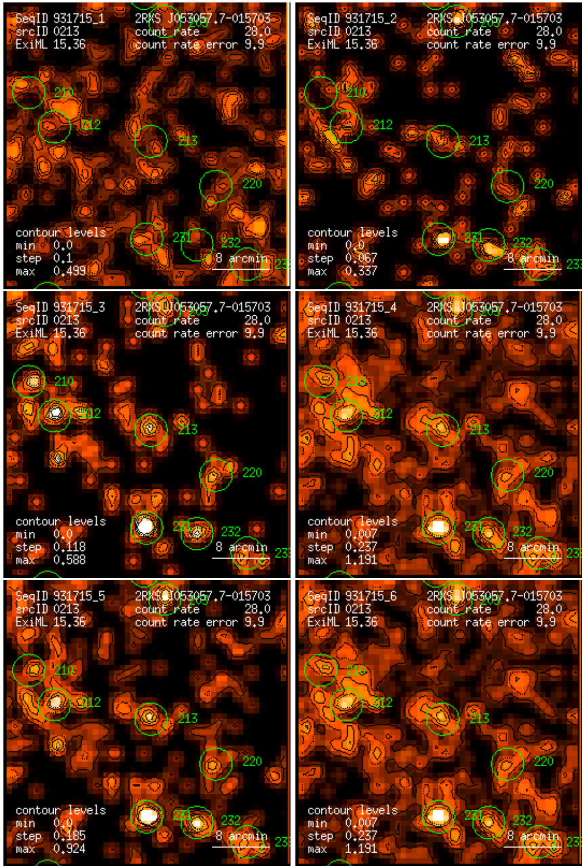
Figure 213: RASS 931715: detection 0213: band rate images, Gaussian filter: (1) PSPC channels 11 – 41, (2) 52 – 90, (3) 91 – 201, (4) 11 – 235, (5) 52 – 201, (6) 11 – 201. Broad band rates in counts/ks. Band rate contour levels in counts/ks/arcmin 2 .
