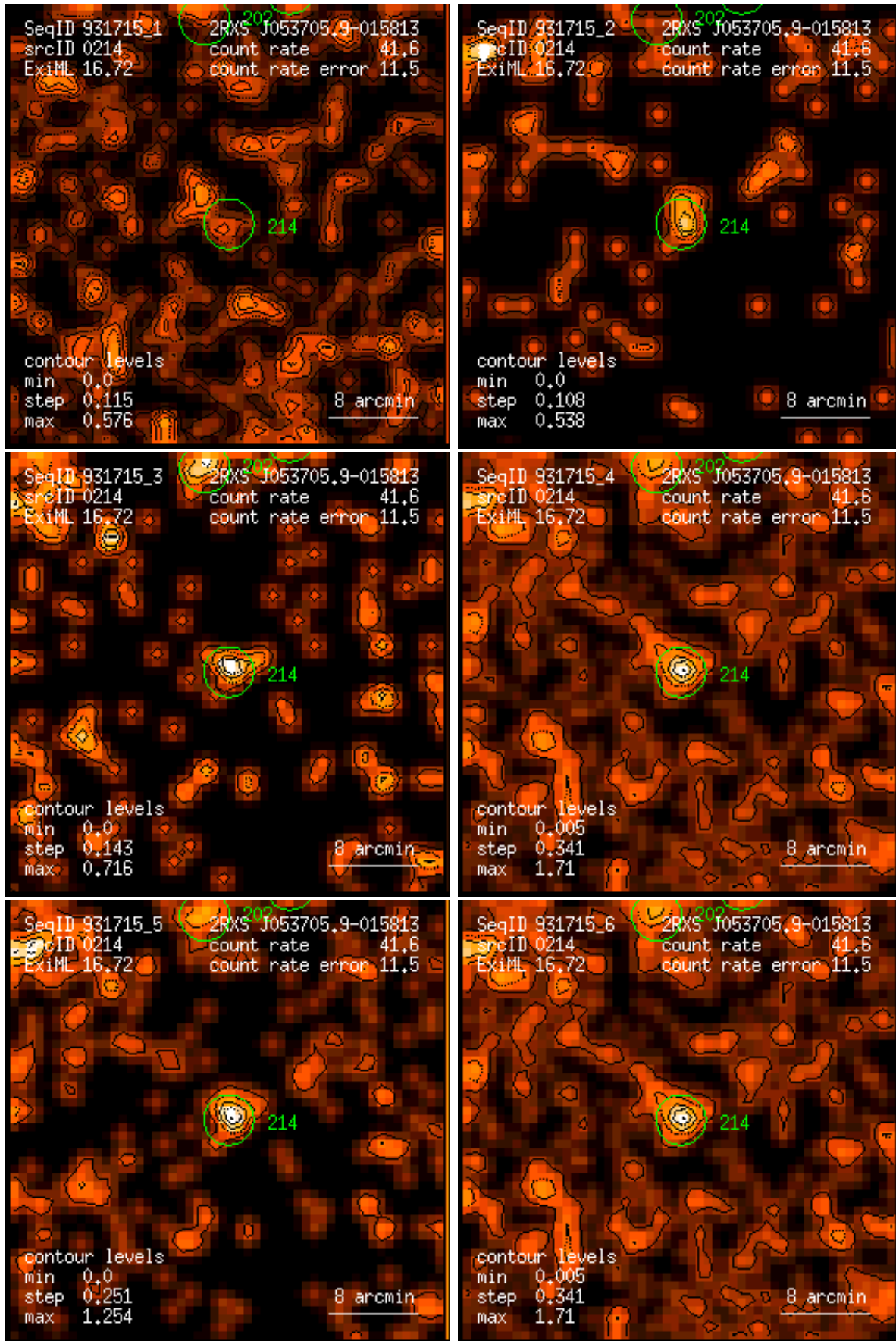
Figure 214: RASS 931715: detection 0214: band rate images, Gaussian filter: (1) PSPC channels 11 – 41, (2) 52 – 90, (3) 91 – 201, (4) 11 – 235, (5) 52 – 201, (6) 11 – 201. Broad band rates in counts/ks. Band rate contour levels in counts/ks/arcmin 2 .
