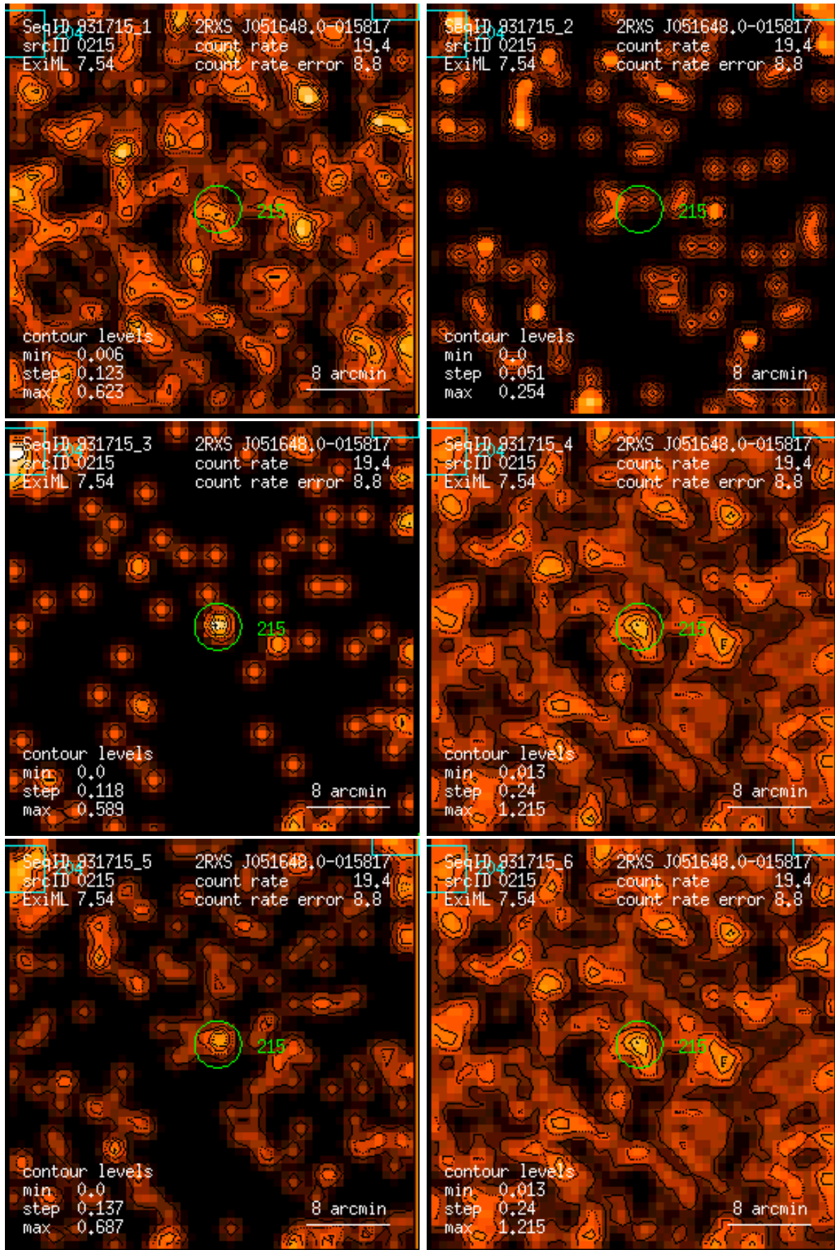
Figure 215: RASS 931715: detection 0215: band rate images, Gaussian filter: (1) PSPC channels 11 – 41, (2) 52 – 90, (3) 91 – 201, (4) 11 – 235, (5) 52 – 201, (6) 11 – 201. Broad band rates in counts/ks. Band rate contour levels in counts/ks/arcmin 2 .
