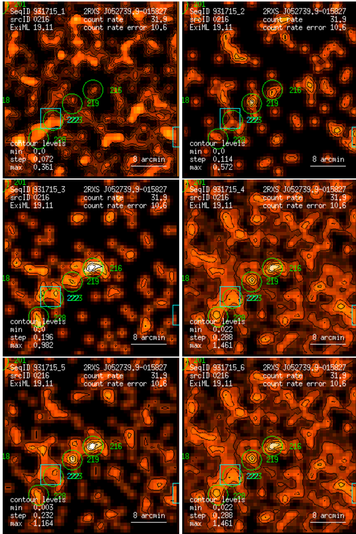
Figure 216: RASS 931715: detection 0216: band rate images, Gaussian filter: (1) PSPC channels 11 – 41, (2) 52 – 90, (3) 91 – 201, (4) 11 – 235, (5) 52 – 201, (6) 11 – 201. Broad band rates in counts/ks. Band rate contour levels in counts/ks/arcmin 2 .
