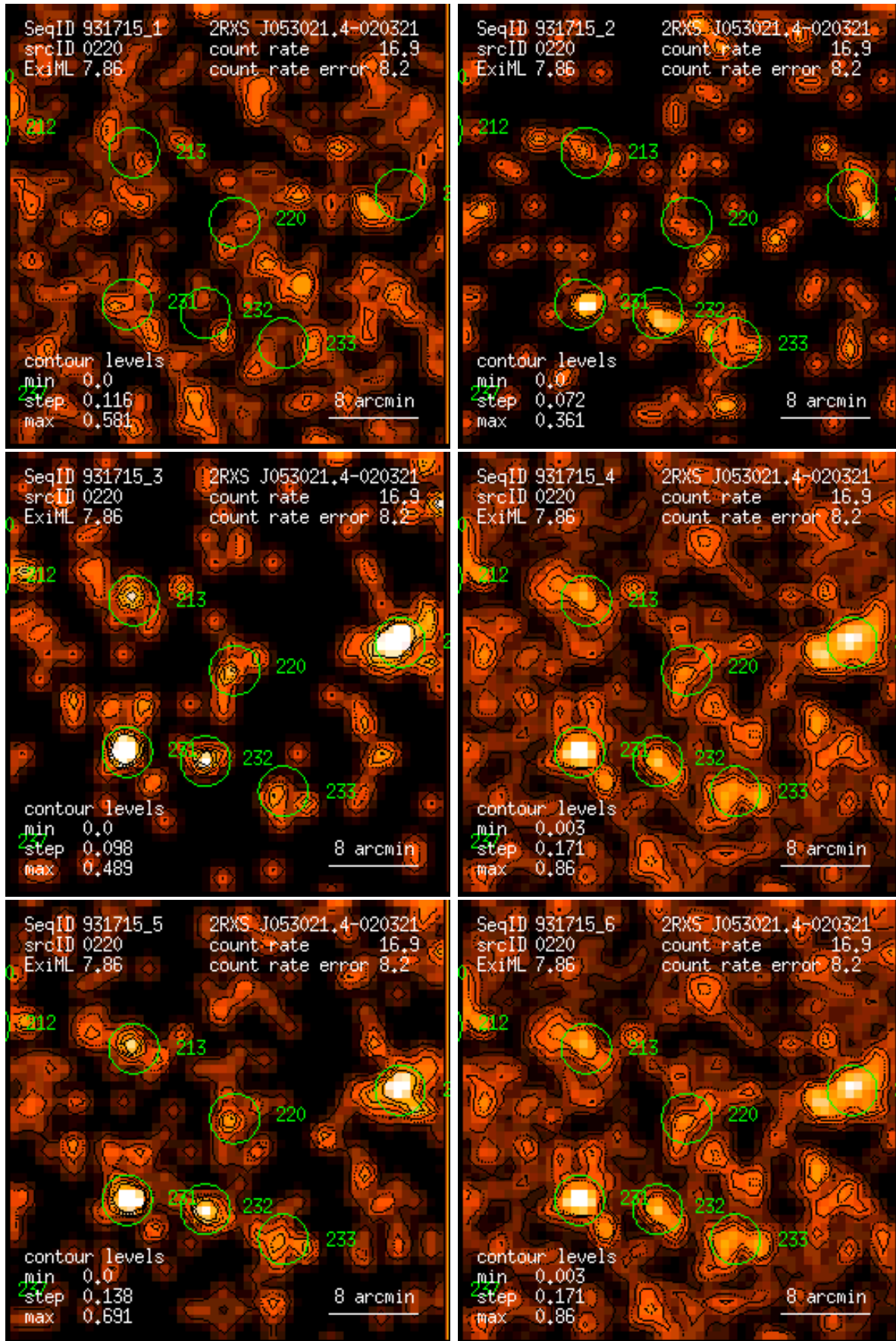
Figure 220: RASS 931715: detection 0220: band rate images, Gaussian filter: (1) PSPC channels 11 – 41, (2) 52 – 90, (3) 91 – 201, (4) 11 – 235, (5) 52 – 201, (6) 11 – 201. Broad band rates in counts/ks. Band rate contour levels in counts/ks/arcmin 2 .
