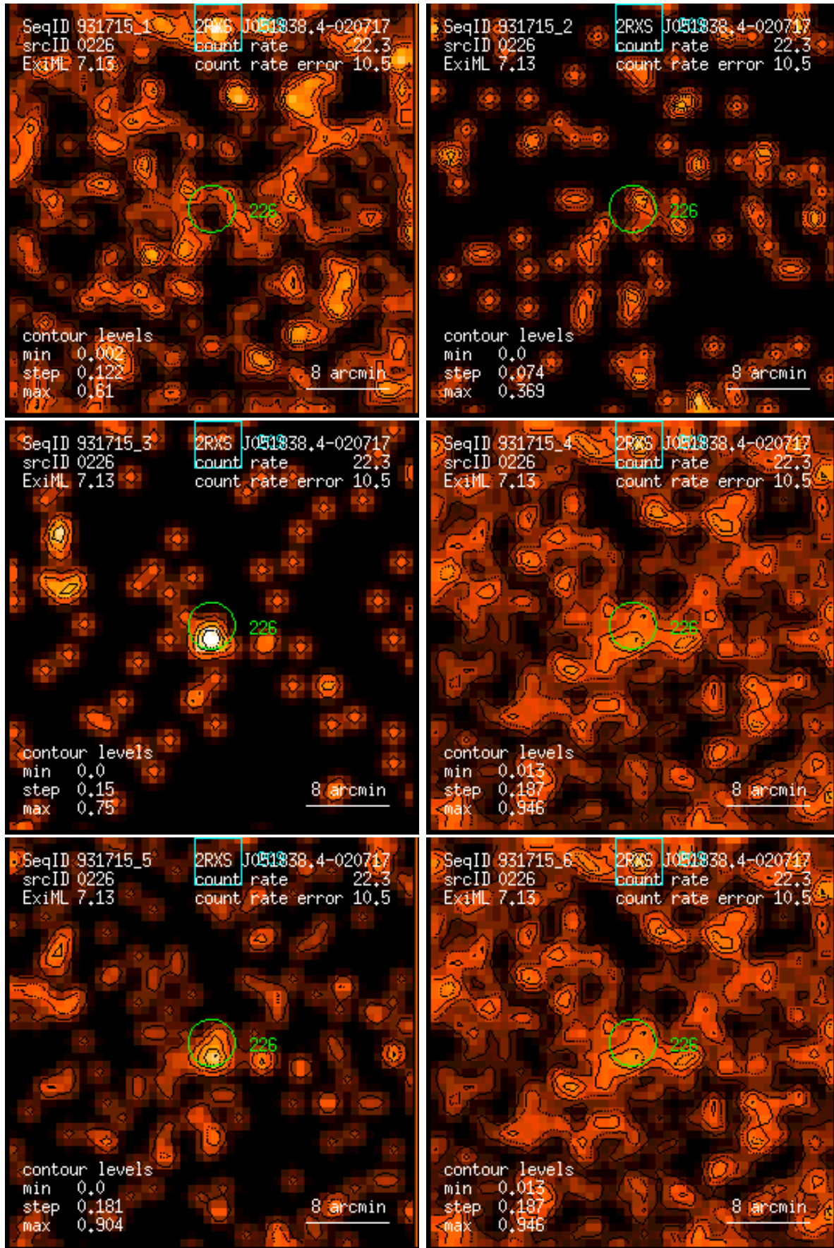
Figure 226: RASS 931715: detection 0226: band rate images, Gaussian filter: (1) PSPC channels 11 – 41, (2) 52 – 90, (3) 91 – 201, (4) 11 – 235, (5) 52 – 201, (6) 11 – 201. Broad band rates in counts/ks. Band rate contour levels in counts/ks/arcmin 2 .
