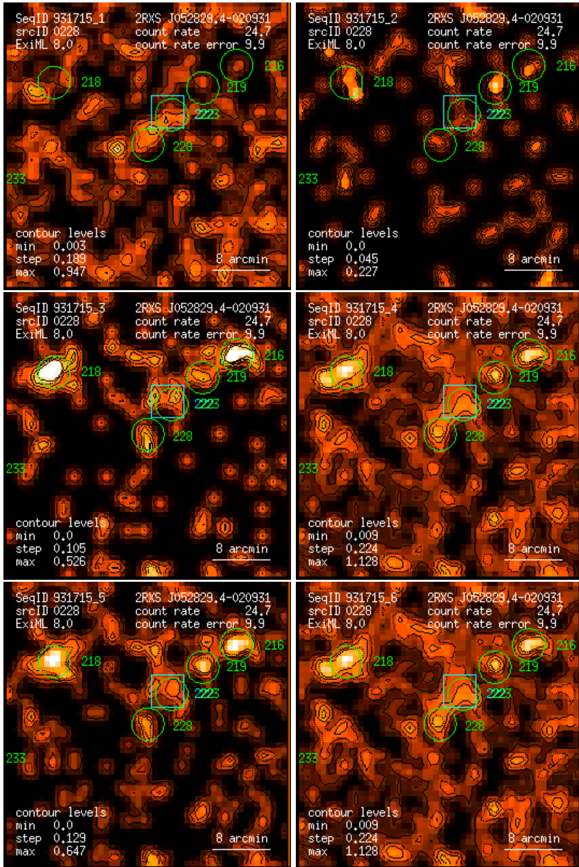
Figure 228: RASS 931715: detection 0228: band rate images, Gaussian filter: (1) PSPC channels 11 – 41, (2) 52 – 90, (3) 91 – 201, (4) 11 – 235, (5) 52 – 201, (6) 11 – 201. Broad band rates in counts/ks. Band rate contour levels in counts/ks/arcmin 2 .
