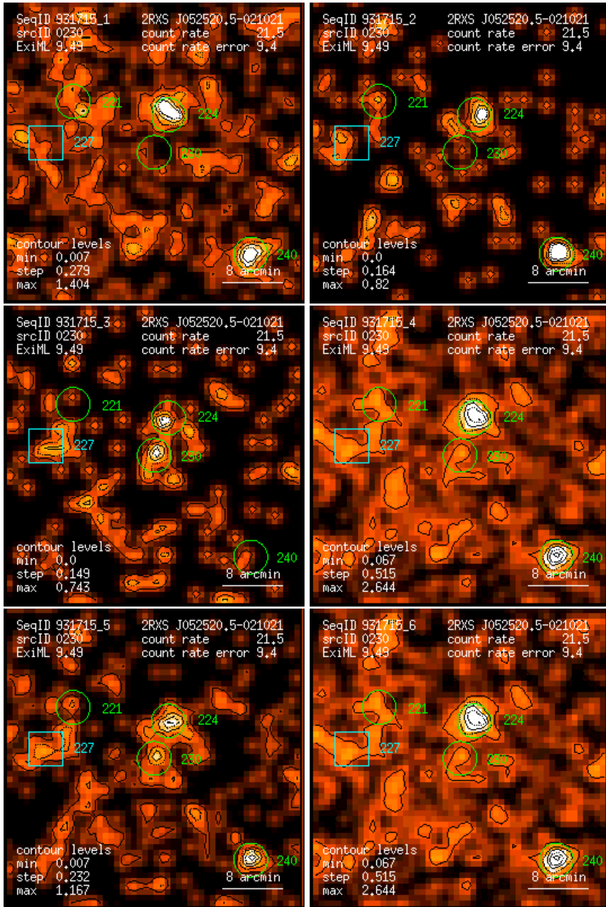
Figure 230: RASS 931715: detection 0230: band rate images, Gaussian filter: (1) PSPC channels 11 – 41, (2) 52 – 90, (3) 91 – 201, (4) 11 – 235, (5) 52 – 201, (6) 11 – 201. Broad band rates in counts/ks. Band rate contour levels in counts/ks/arcmin 2 .
