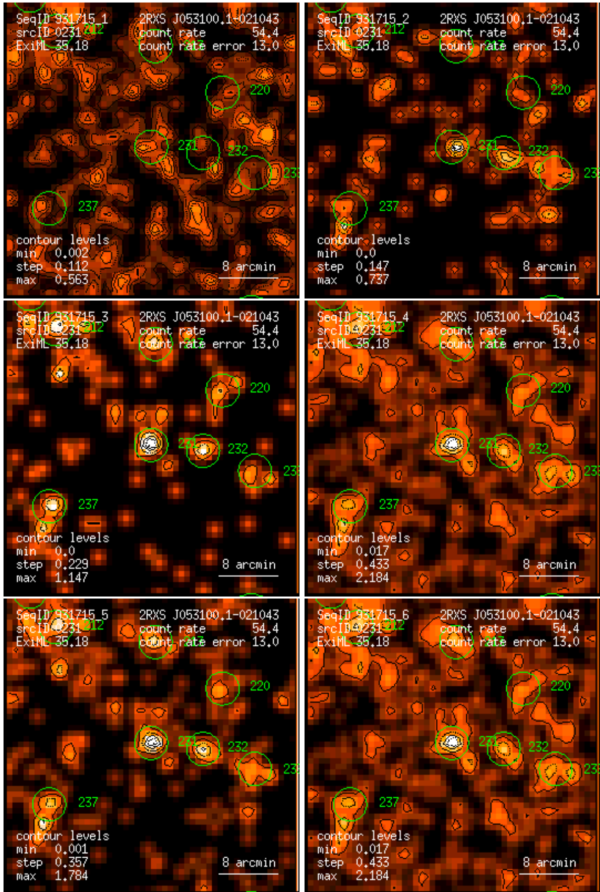
Figure 231: RASS 931715: detection 0231: band rate images, Gaussian filter: (1) PSPC channels 11 – 41, (2) 52 – 90, (3) 91 – 201, (4) 11 – 235, (5) 52 – 201, (6) 11 – 201. Broad band rates in counts/ks. Band rate contour levels in counts/ks/arcmin 2 .
